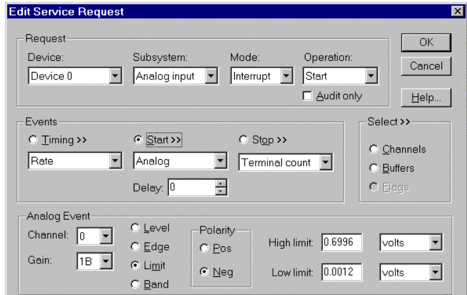
How to set up the DAS-800 Series for post-triggered analog input.
