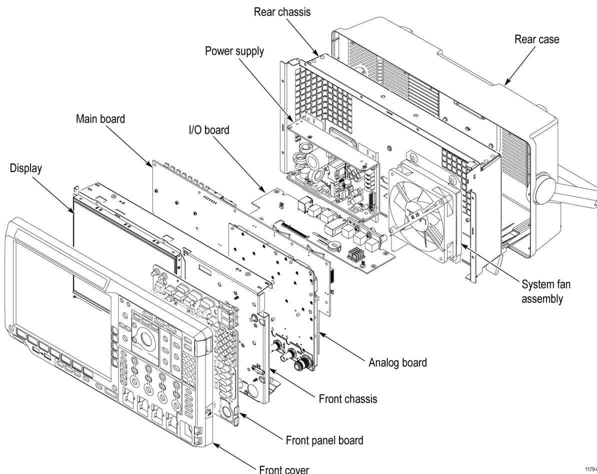
Figure 3: Module locator
