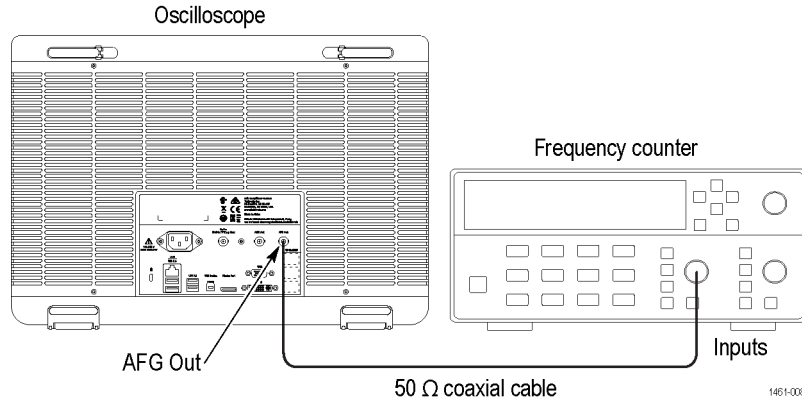
Figure 1: Frequency/period test
