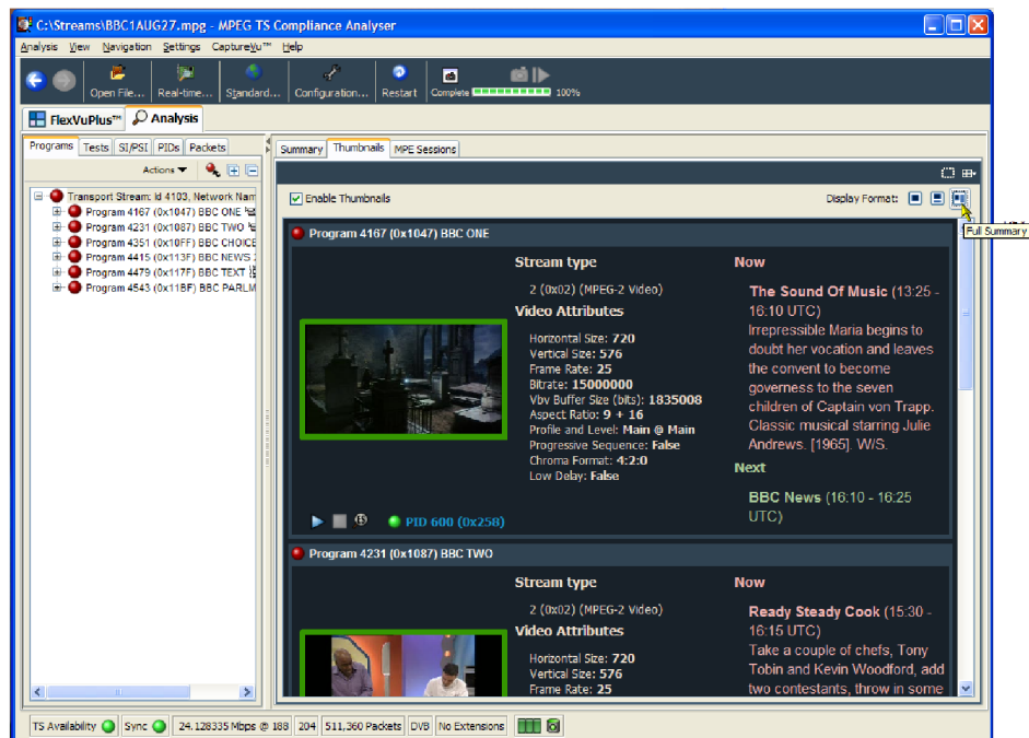
Figure 1-52: Now Playing - Detail view
