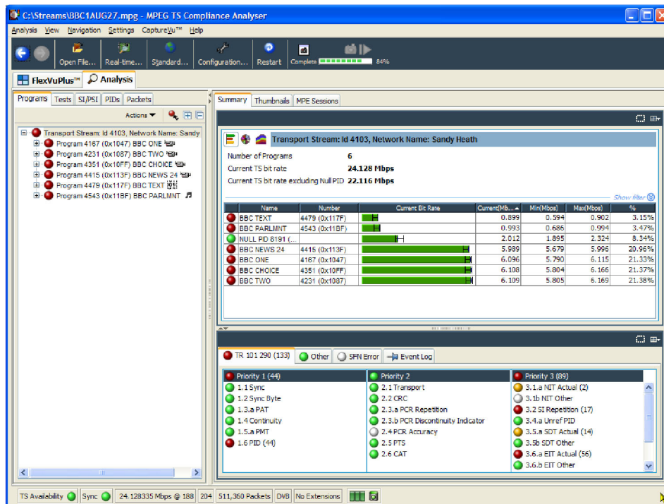
Figure 1-12: TSCA window showing analysis progress
