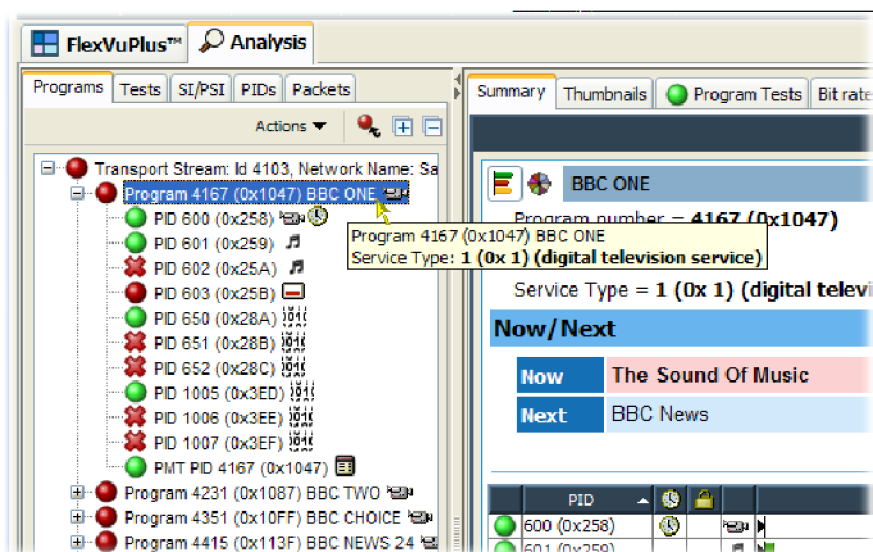
Figure 1-77: PID count
