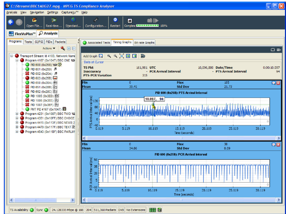
Figure 1-45: Timing graphs
