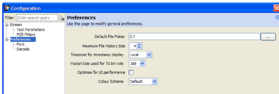
Figure 1-71: Configuration - Preferences
