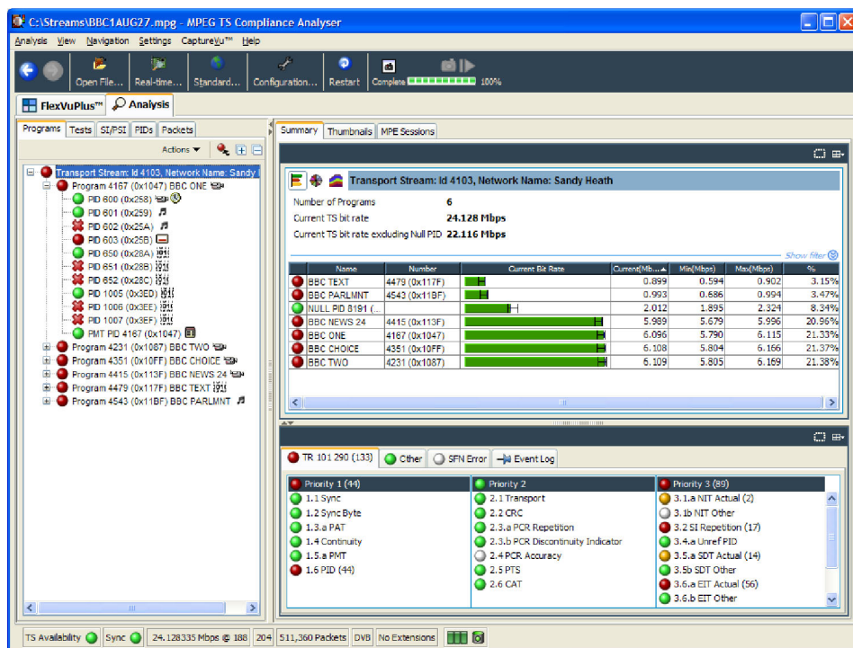
Figure 1-18: Program view
