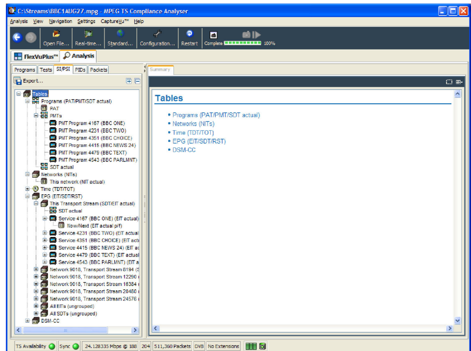
Figure 1-27: Tables view
