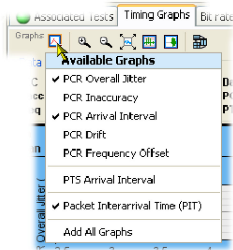
Figure 1-46: Graph toolbar
