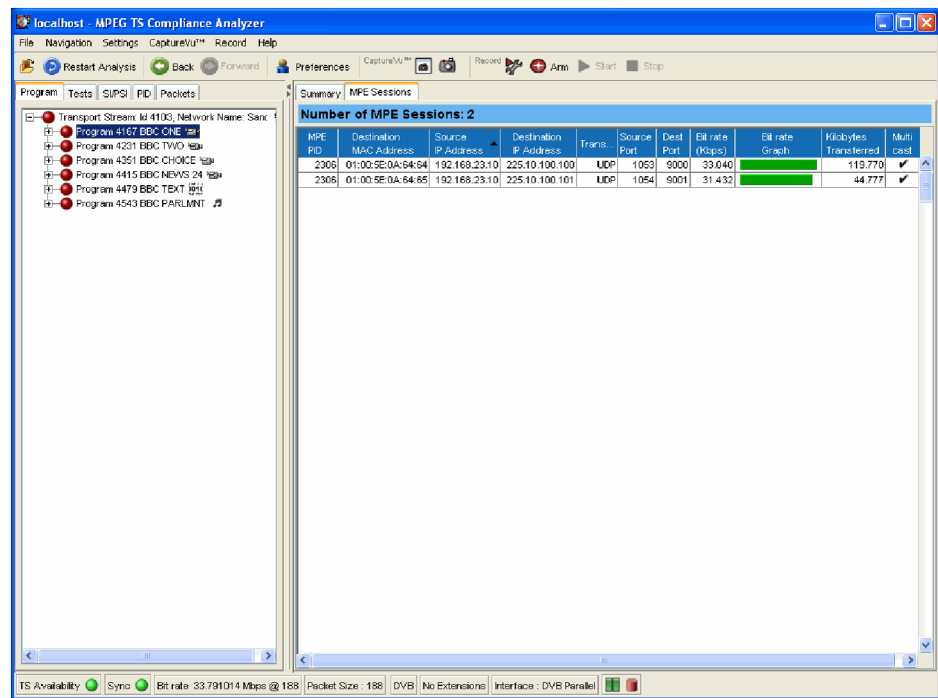
Figure 1-64: MPE view
