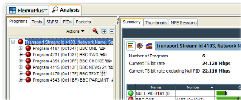
Figure 1-76: Program count
