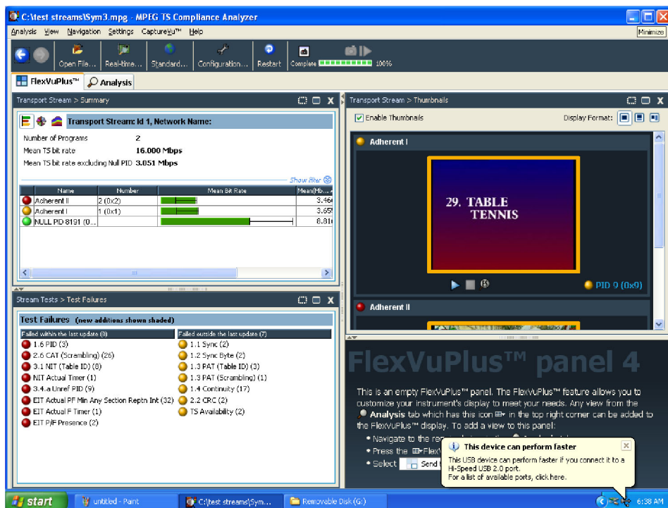
Figure 1-14: FlexVuPlus window
