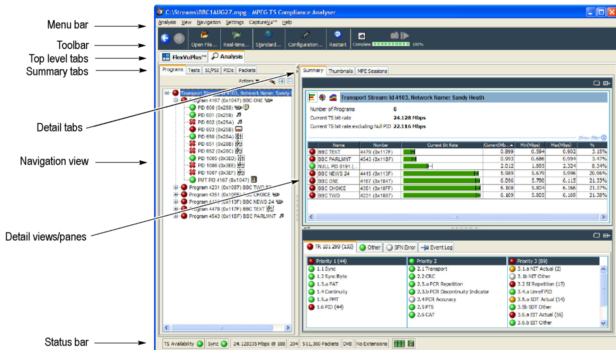
Figure 1-15: Analyzer window
