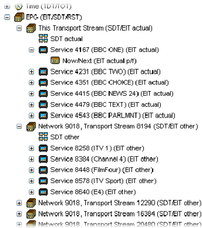
Figure 1-63: EPG nodes
