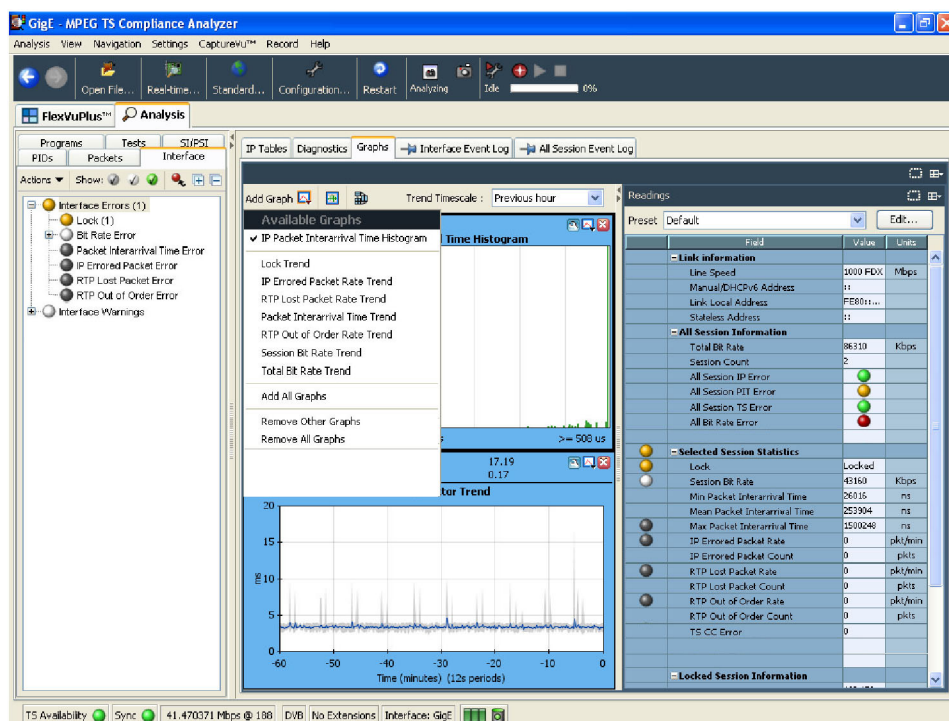
Figure 1-41: IP Video interface graphs (tear-off view)
