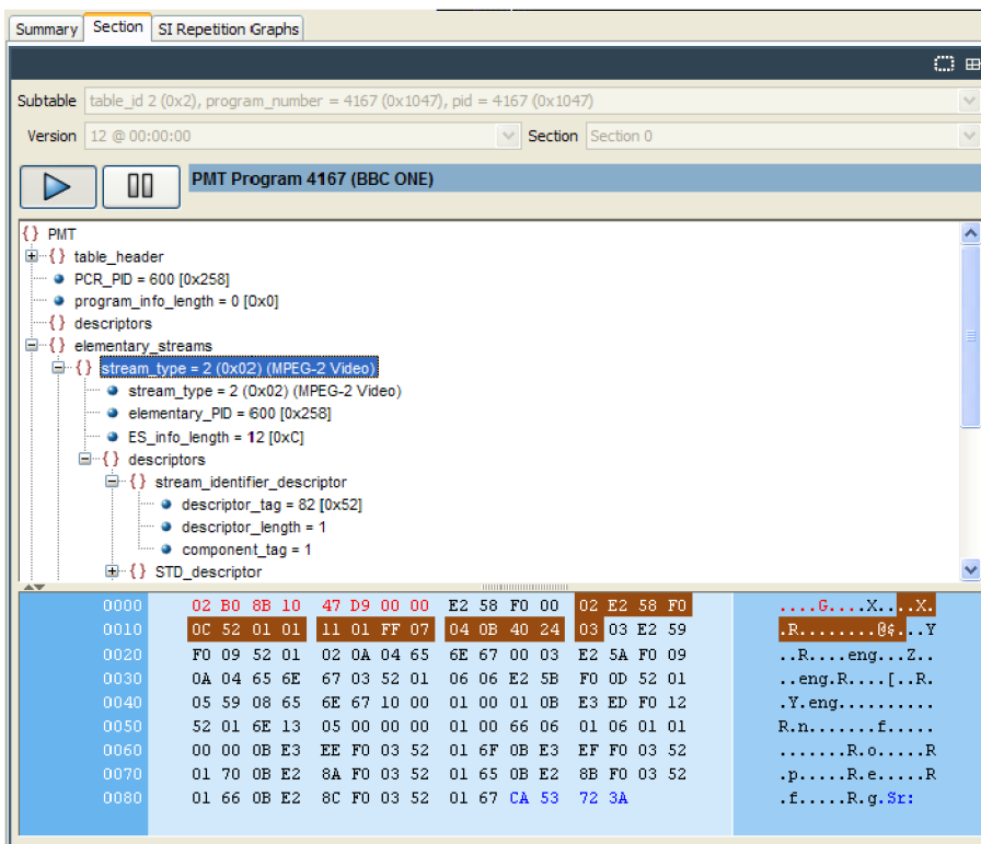
Figure 1-29: Section payload
