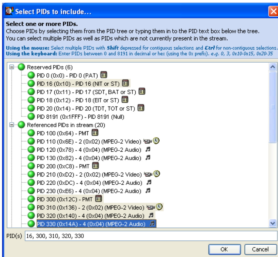
Figure 1-67: PID selection
