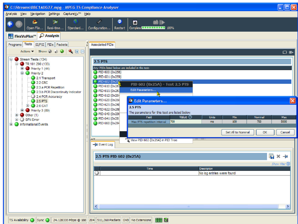
Figure 1-54: PID test parameters
