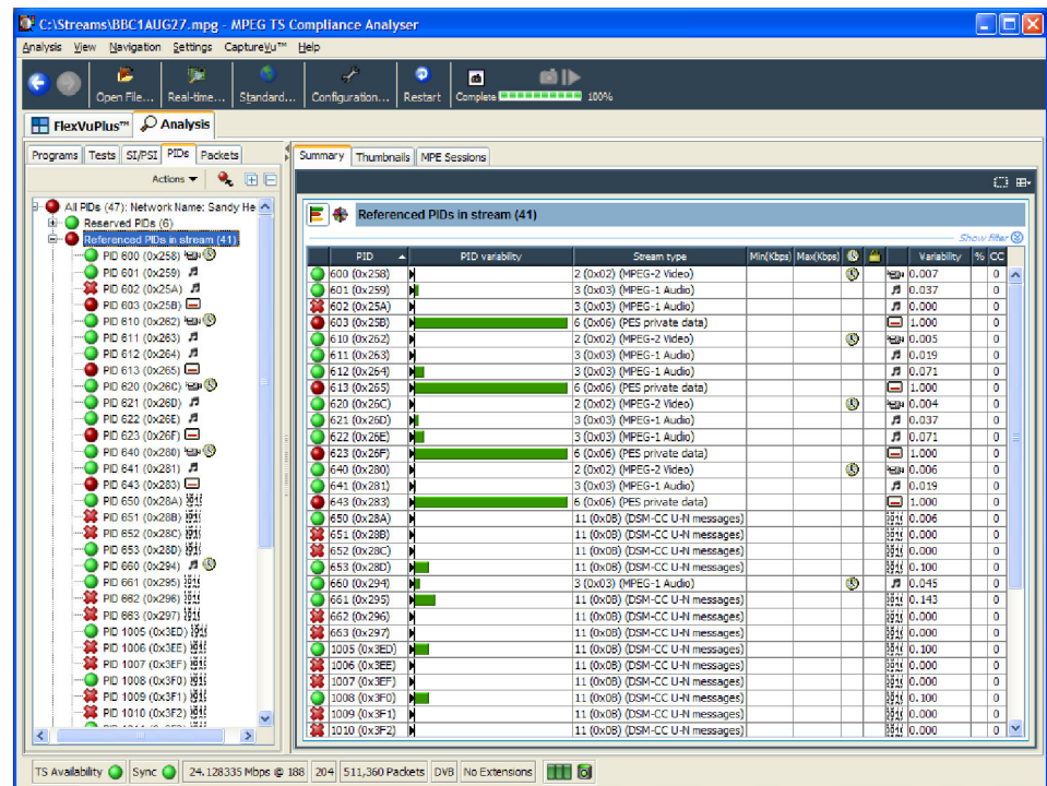
Figure 1-31: PID Information view
