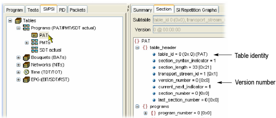
Figure 1-82: Table Identity and Version (section view)
