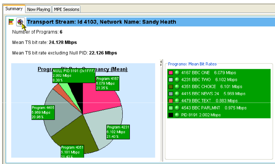
Figure 1-61: Pie chart
