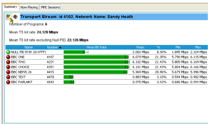
Figure 1-60: Bar chart
