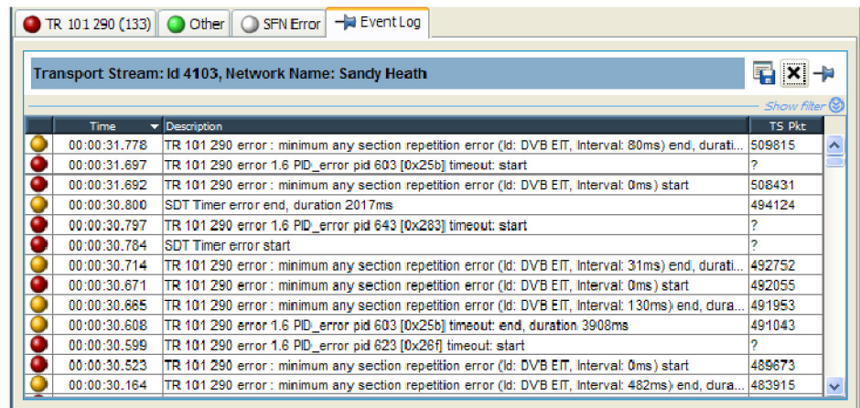
Figure 1-21: Event log
