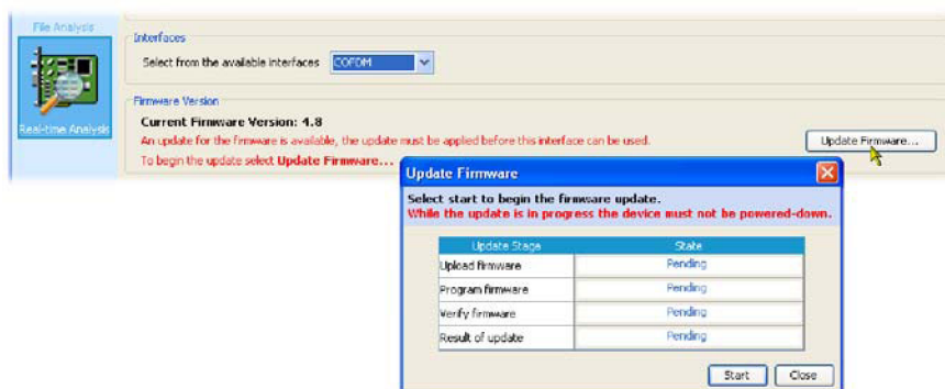
Figure 1-8: Firmware update
