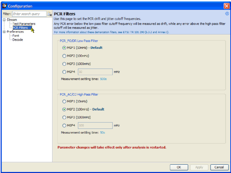
Figure 1-70: Configuration - PCR Filters
