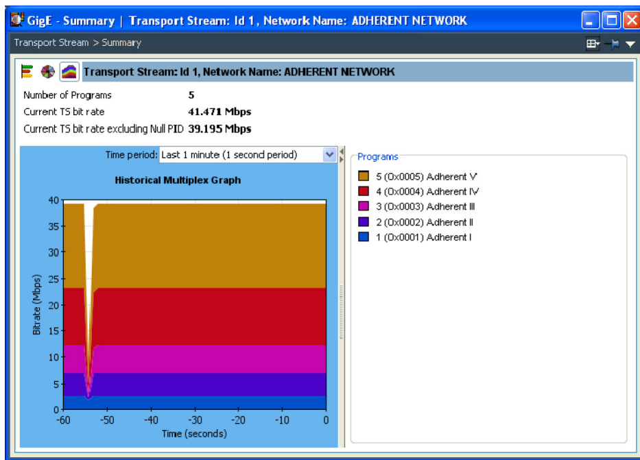
Figure 1-20: Historical Multiplex Graph
