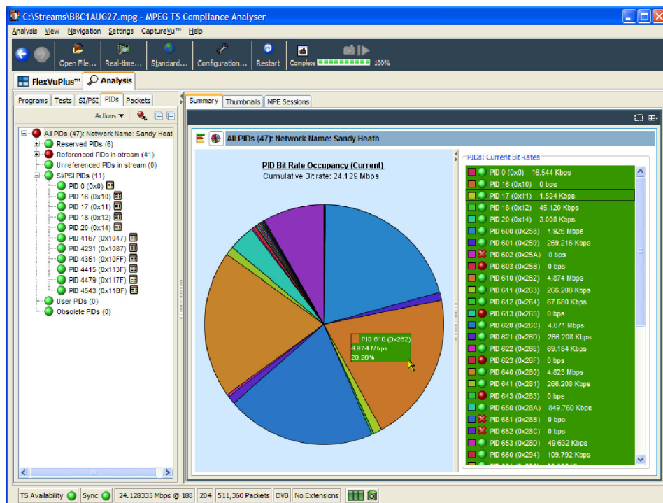
Figure 1-30: PID Summary view
