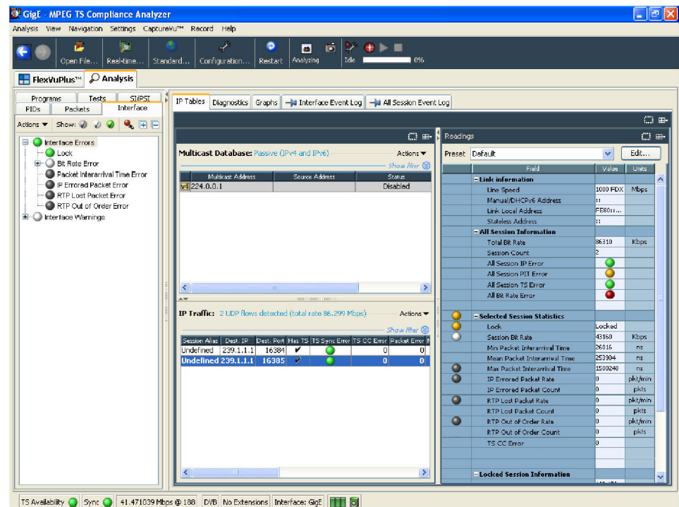
Figure 1-37: Interface view - IP Video
