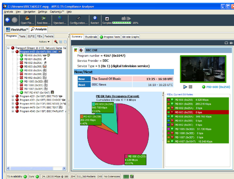
Figure 1-79: Program PID bit rate - pie chart
