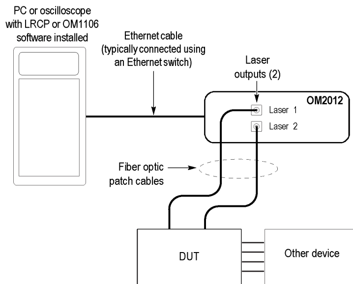
Figure 1: OM2012 connection diagram
