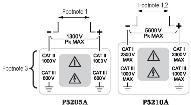
Figure 2: Specification table footnotes referring to the probe input limits on the P5205A and P5210A probes
