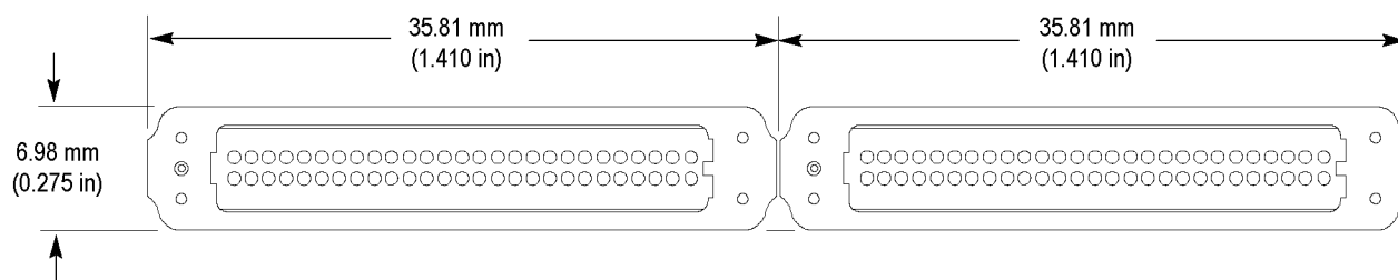
Figure 25: End-to-end layout
