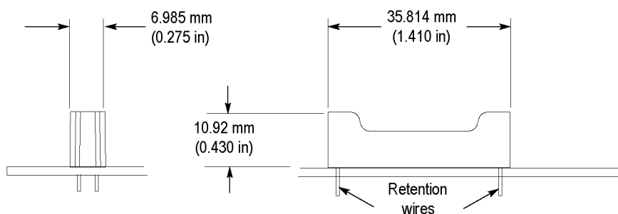
Figure 22: Alternate retention assembly dimensions
