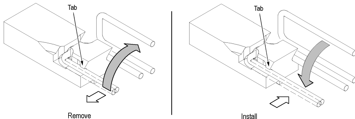
Figure 7: Replacing the wires on the retention posts
