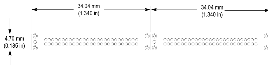
Figure 21: End-to-end layout
