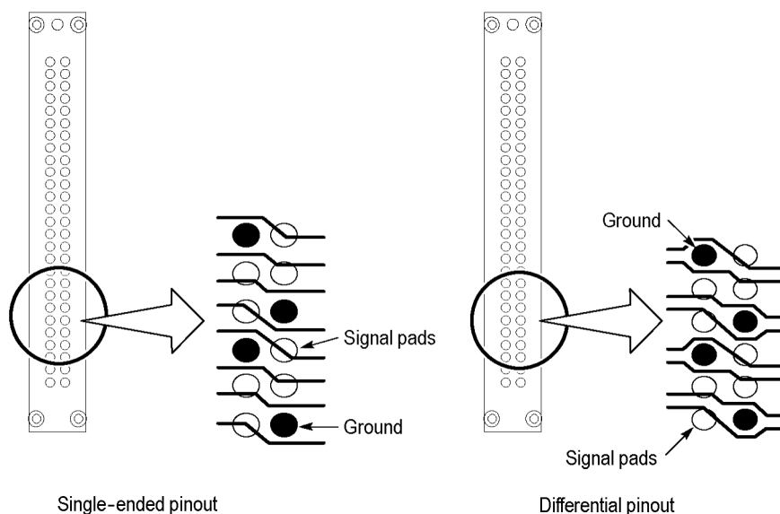
Figure 26: Signal routing on the target system
