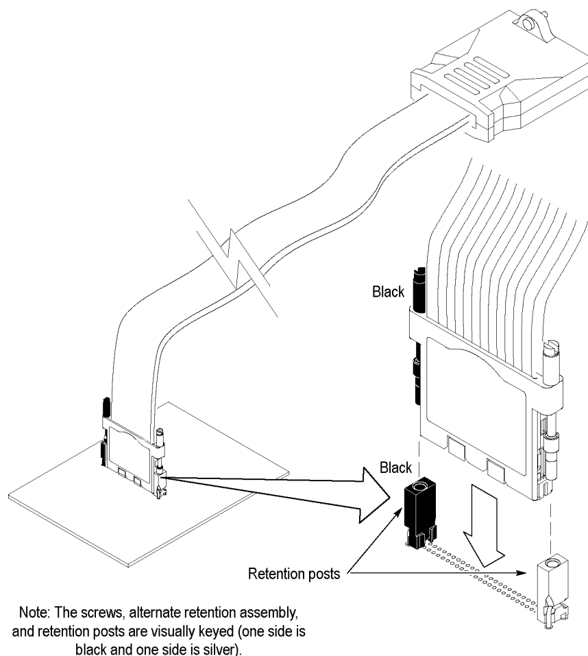
Figure 12: Connecting the probes to the target system
