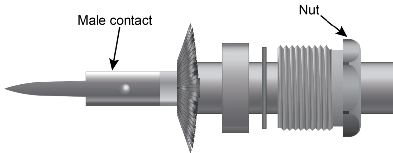
Figure 5: Install the male contact
