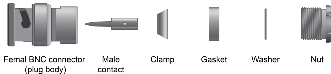
Figure 1: Main assembly parts
