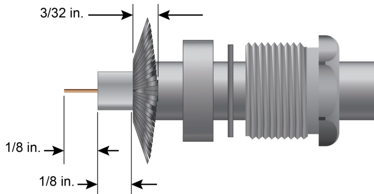
Figure 4: Flare braided wire back
