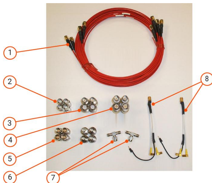
Figure 1: 4200-CVU-PROBER-KIT contents
