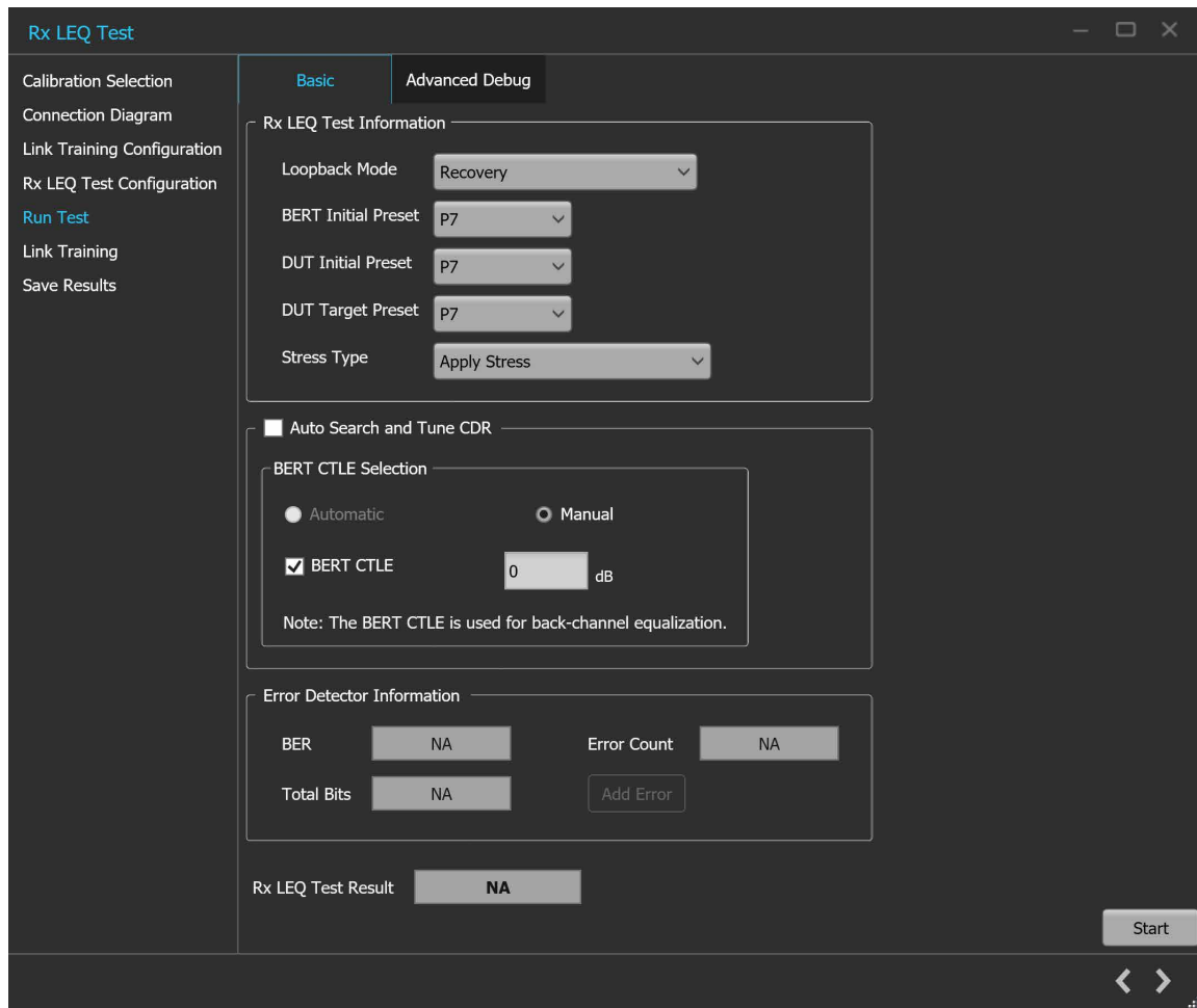
Figure 45: Rx LEQ Test: Run Test (Basic)
