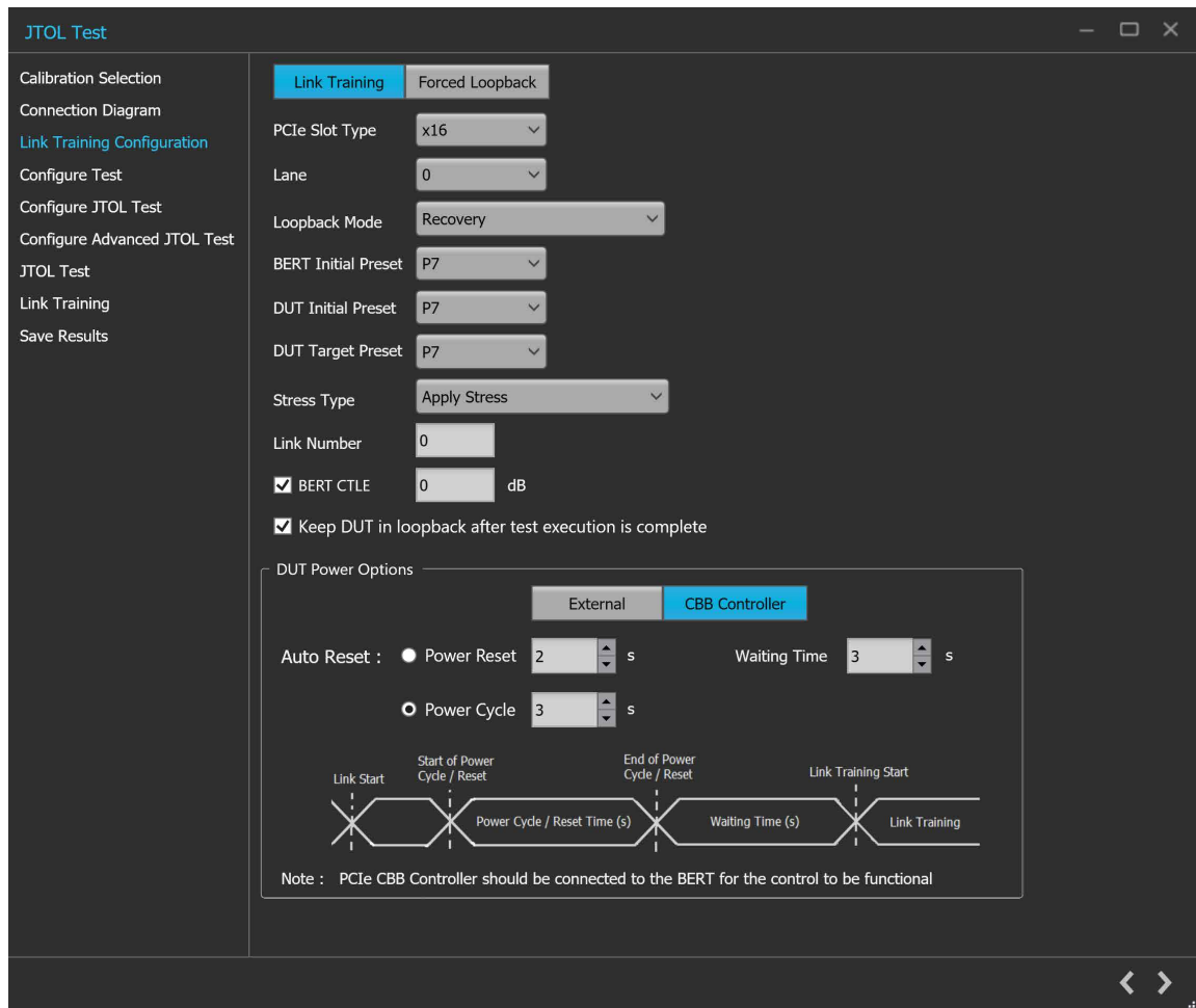
Figure 65: JTOL Test: Link Training Configuration (Link Training-CBB Controller)
