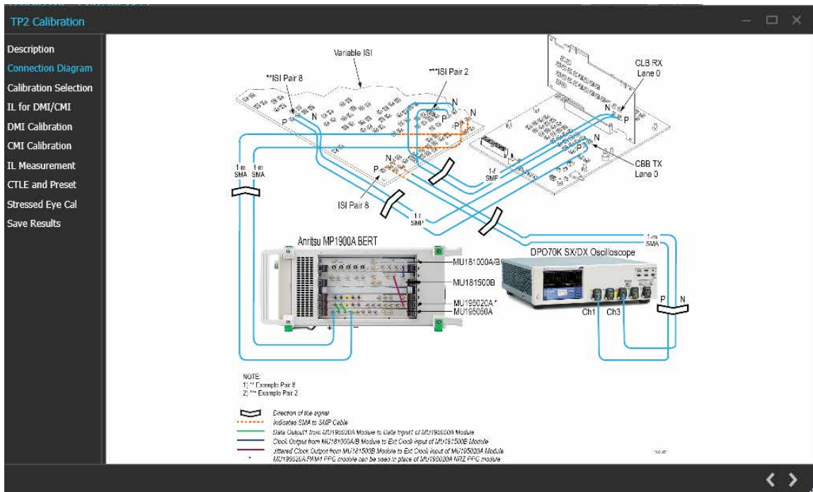
Figure 27: TP2 Calibration: Connection Diagram-System
