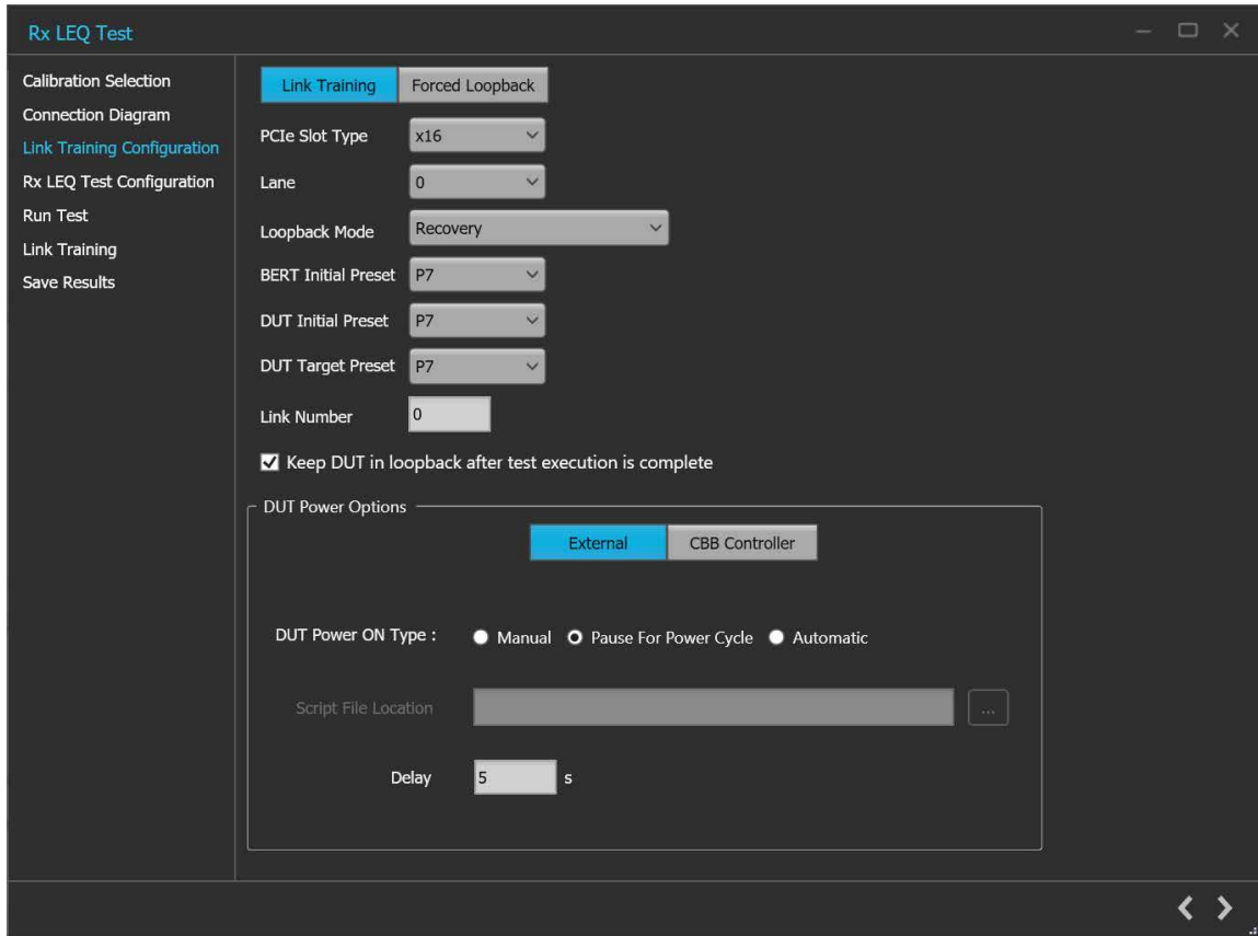
Figure 40: Rx LEQ Test: Link Training Configuration (Link Training-External)
