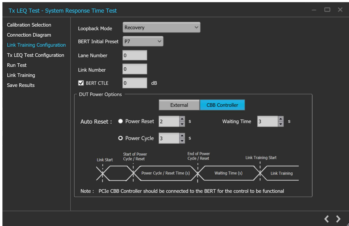
Figure 53: Tx LEQ Test: Link Training Configuration (CBB Controller)
