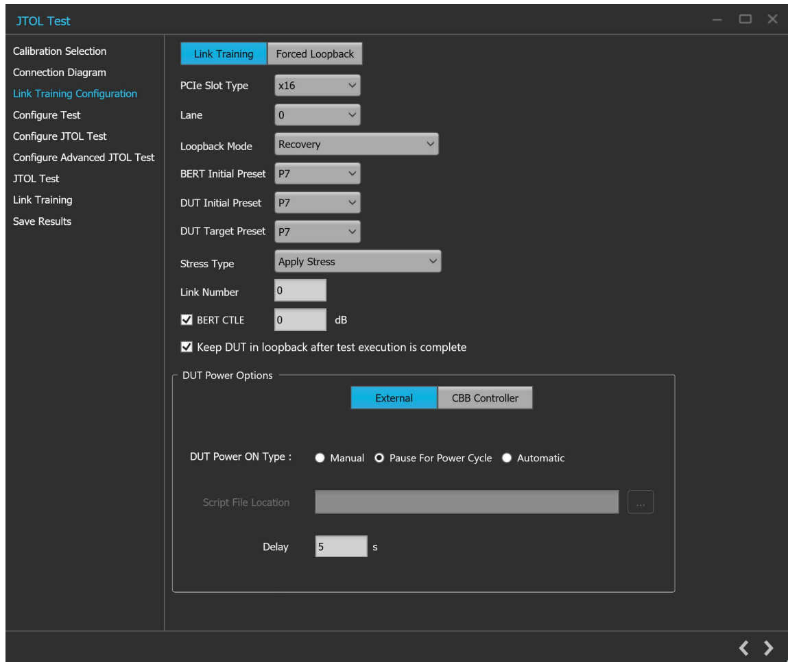
Figure 64: JTOL Test: Link Training Configuration (Link Training-External)
