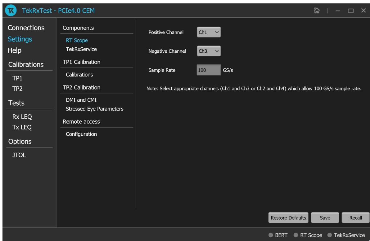
Figure 6: Settings panel
