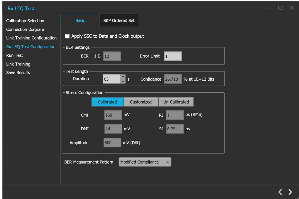
Figure 43: Rx LEQ Test: Rx LEQ Test Configuration (Basic)
