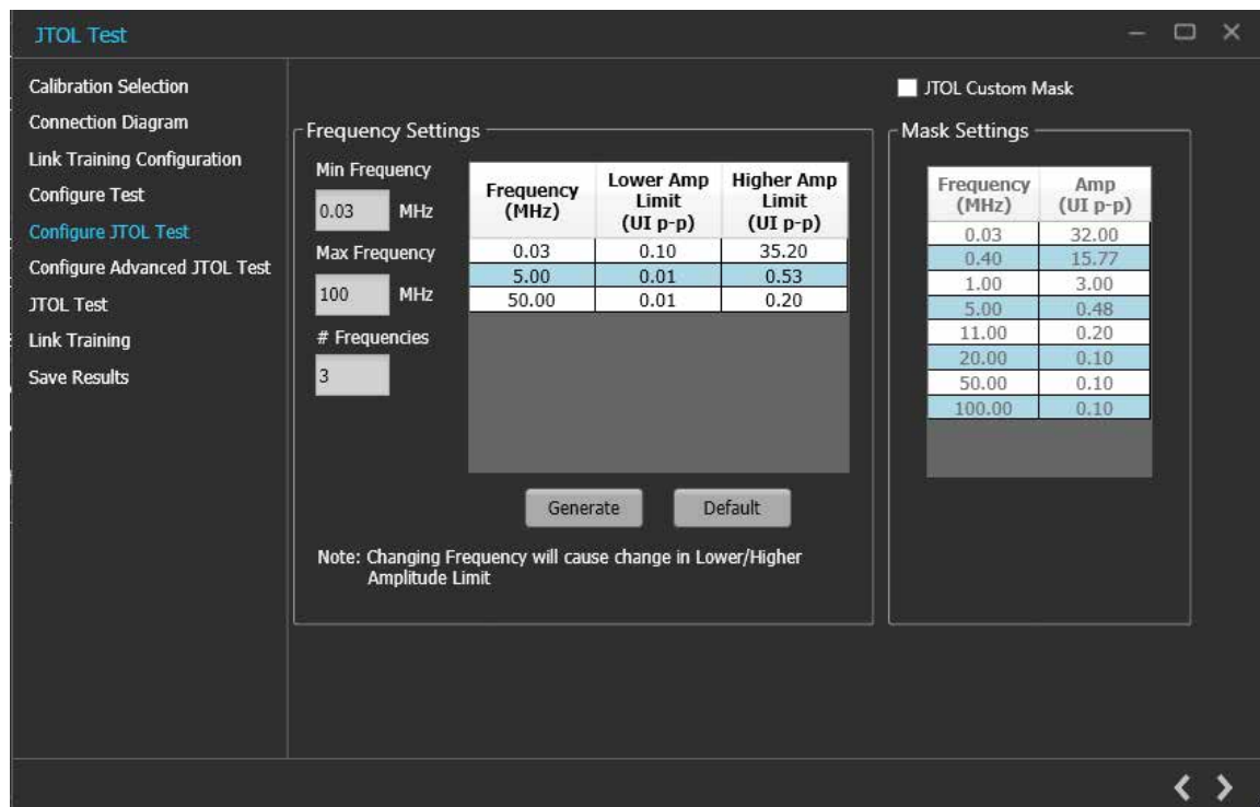
Figure 73: JTOL Test: Configure JTOL Test
