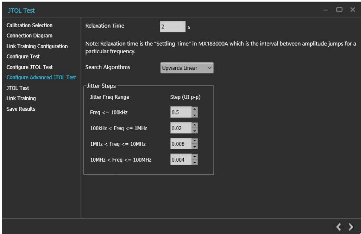
Figure 74: JTOL Test: Configure Advanced JTOL Test
