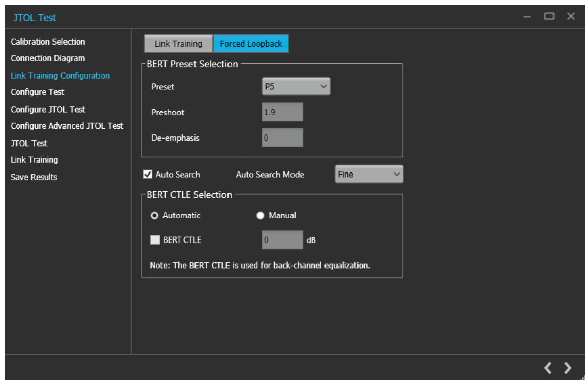
Figure 70: JTOL Test: Link Training Configuration (Forced Loopback)
