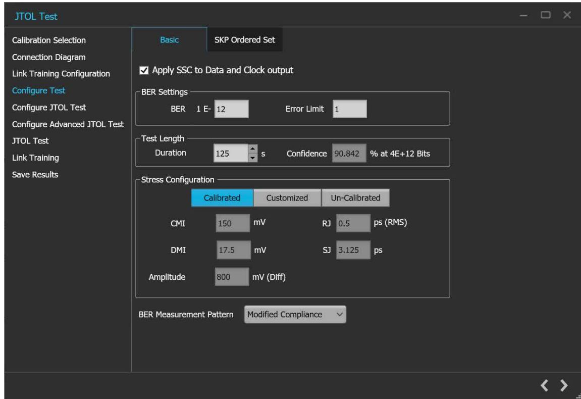
Figure 71: JTOL Test: Configure Test (Basic)
