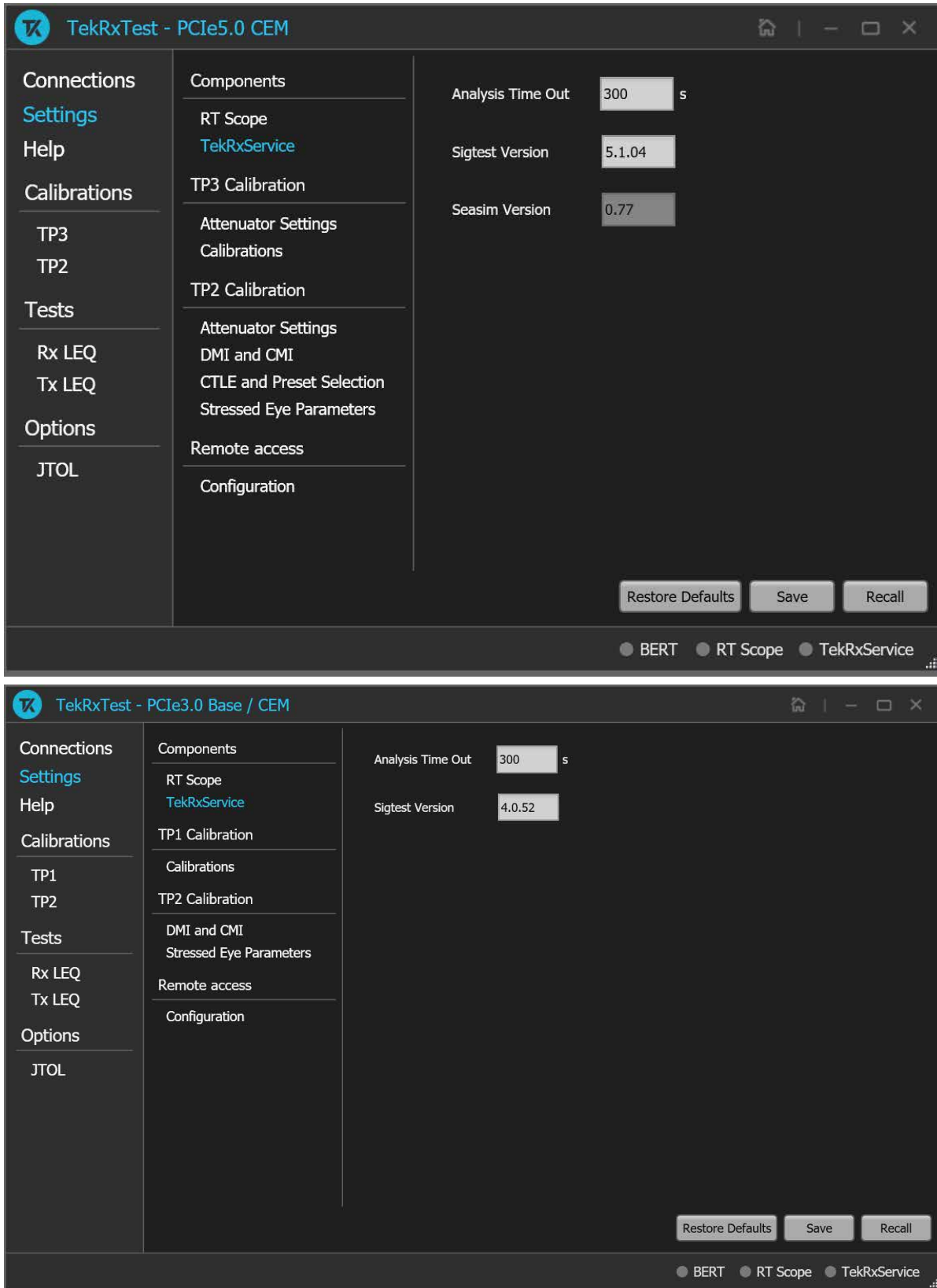
Figure 8: Components: TekRxService
