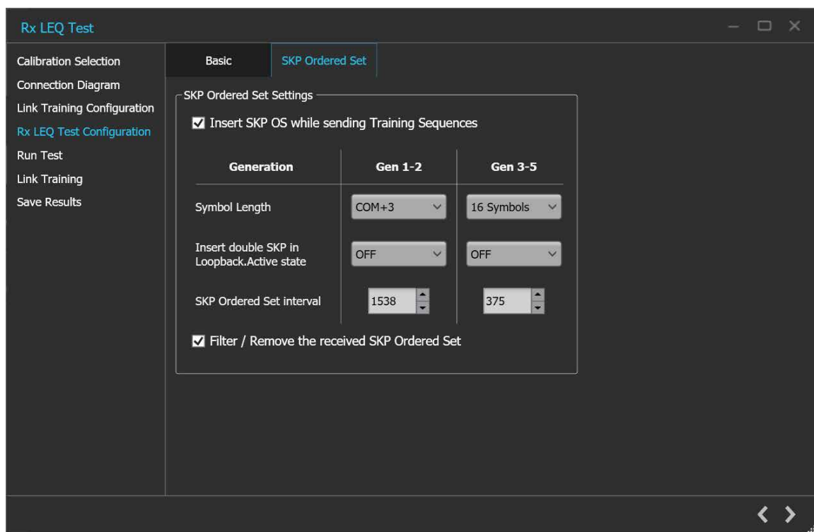
Figure 48: Rx LEQ Test: Rx LEQ Test Configuration (SKP Ordered Set)
