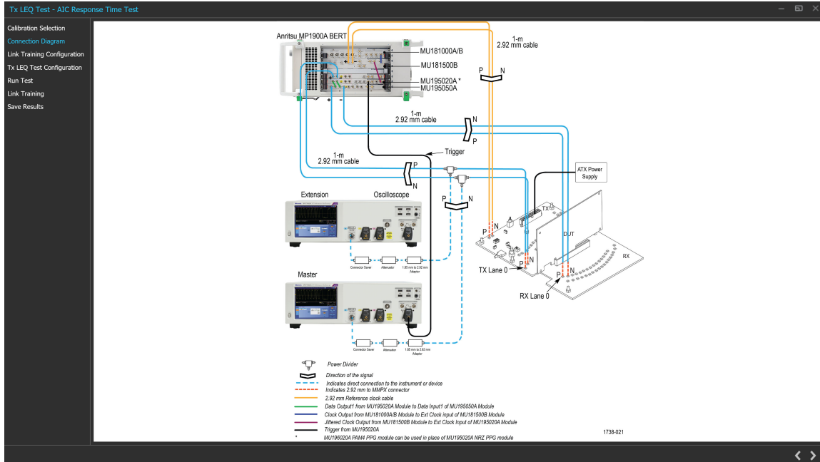
Figure 54: Tx LEQ Test: Connection Diagram(AIC)
