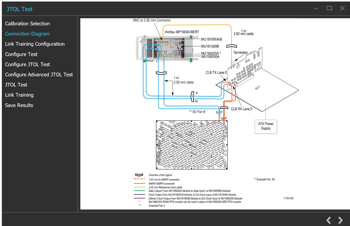
Figure 67: JTOL Test: Connection Diagram(System)
