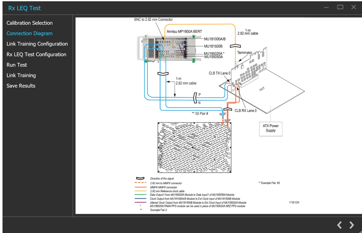
Figure 43: Rx LEQ Test: Connection Diagram(System)
