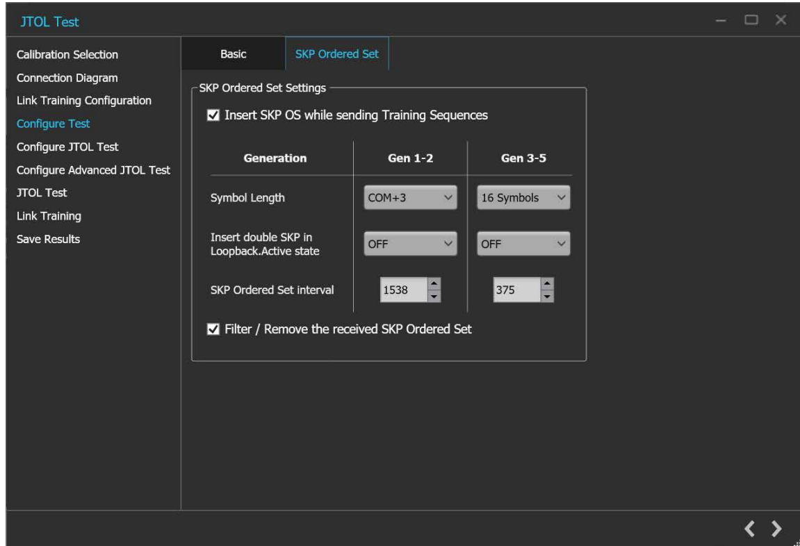
Figure 72: JTOL Test: Configure Test (SKP Ordered Set)
