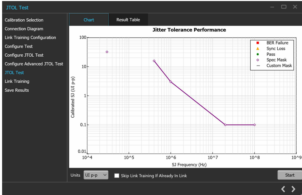
Figure 75: JTOL Test: JTOL Chart
