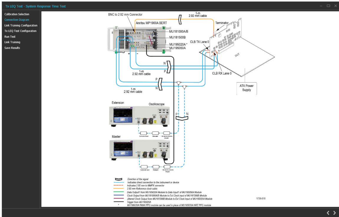
Figure 55: Tx LEQ Test: Connection Diagram(System)
