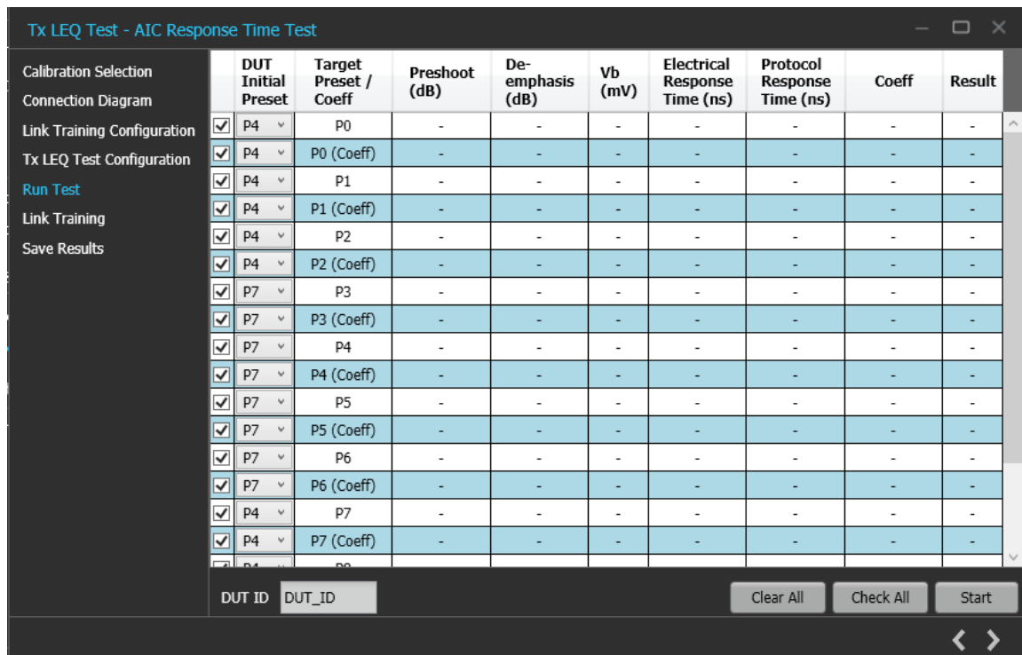
Figure 61: Tx LEQ Test: Run Test(AIC Response Time Test)
