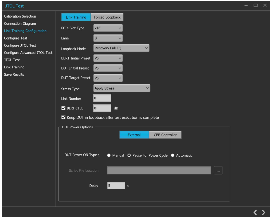
Figure 68: JTOL Test: Link Training Configuration (Link Training-External)
