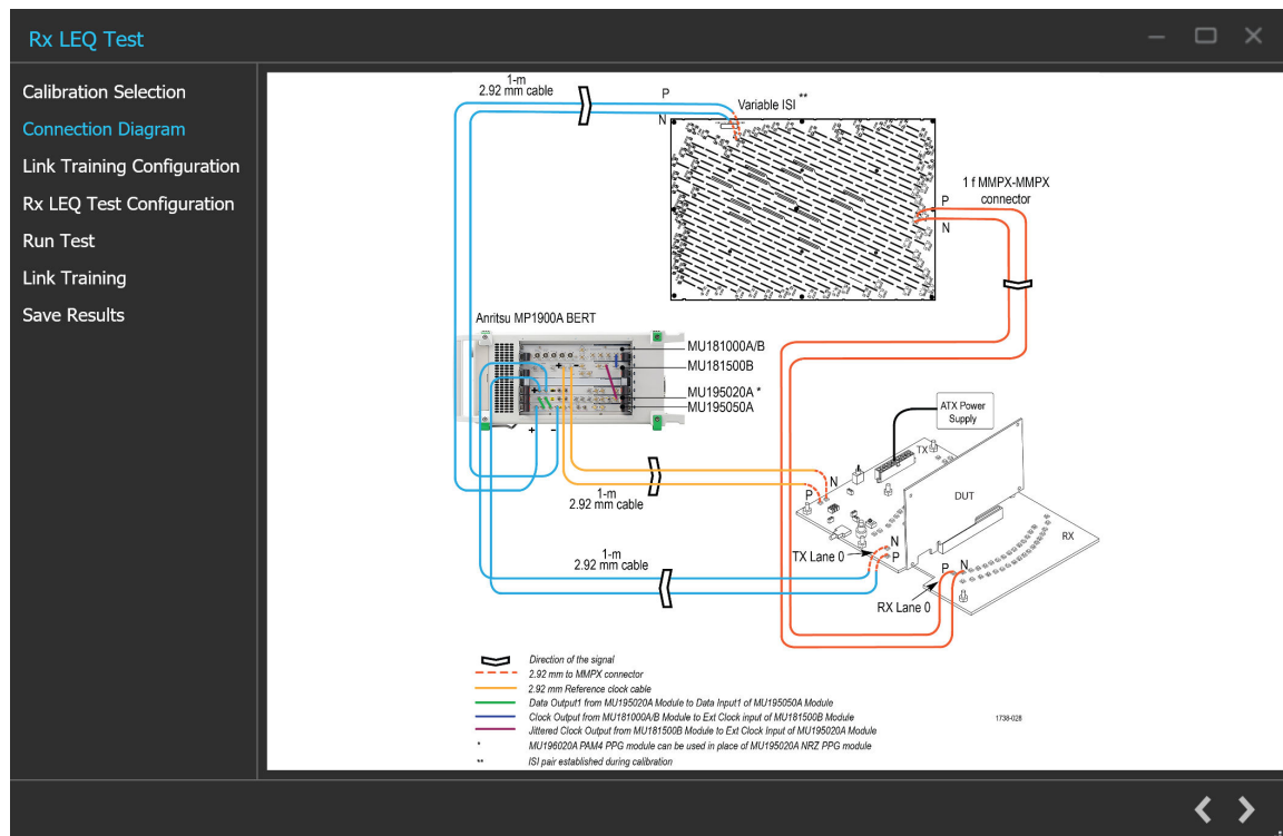
Figure 42: Rx LEQ Test: Connection Diagram(AIC)
