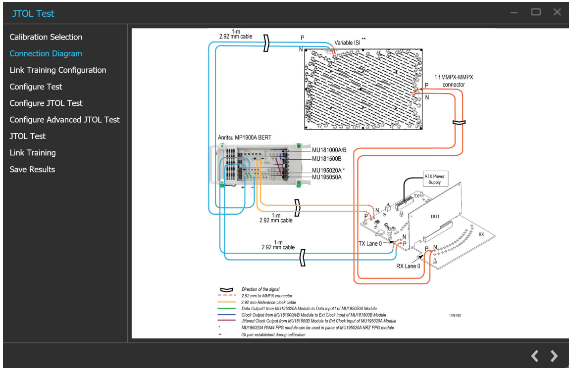
Figure 66: JTOL Test: Connection Diagram(AIC)
