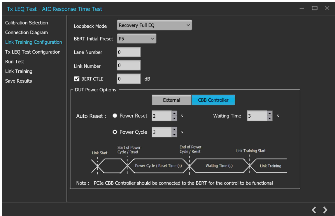
Figure 57: Tx LEQ Test: Link Training Configuration (CBB Controller)
