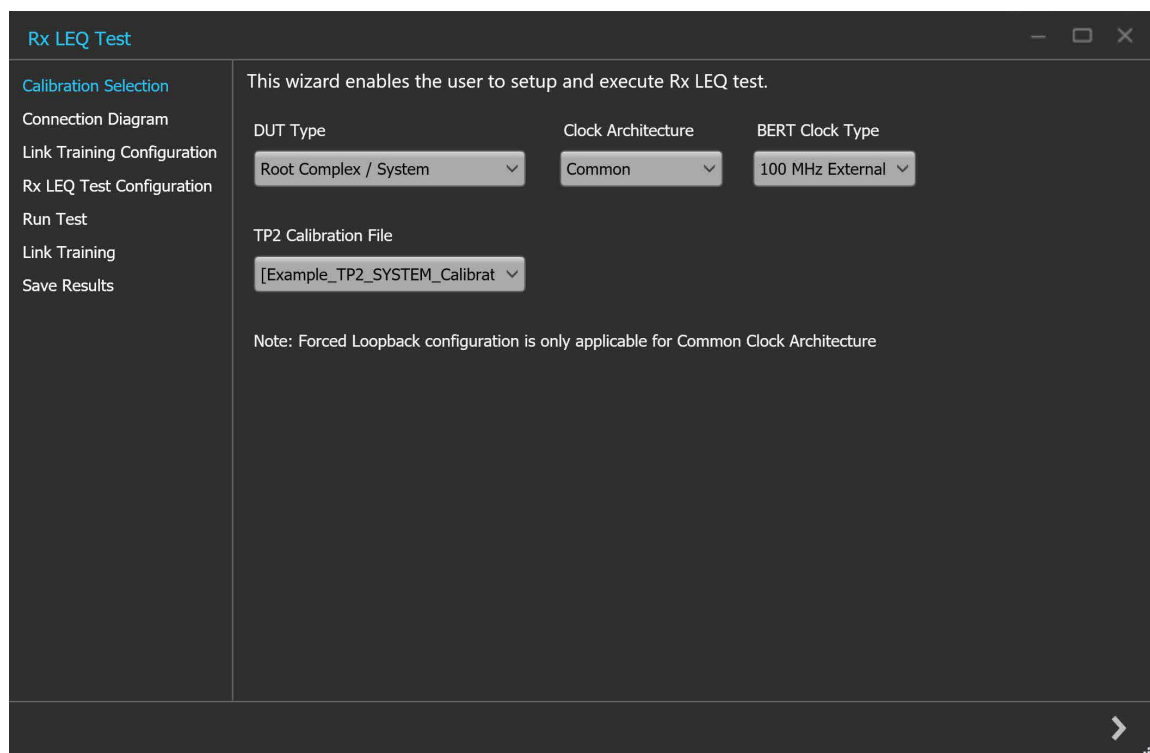
Figure 41: Rx LEQ Test: Calibration Selection
