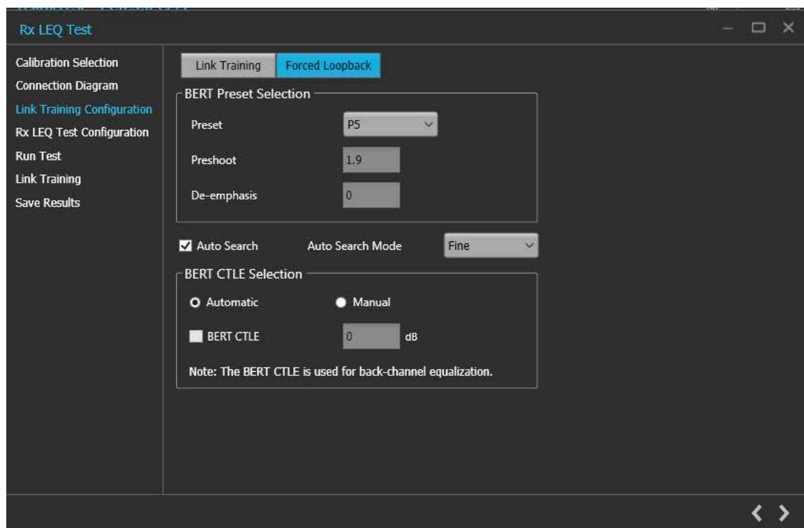
Figure 46: Rx LEQ Test: Link Training Configuration (Forced Loopback)
