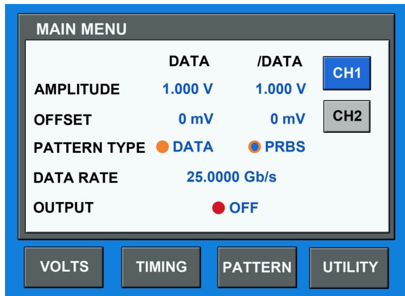
Figure 10: GUI Main menu
