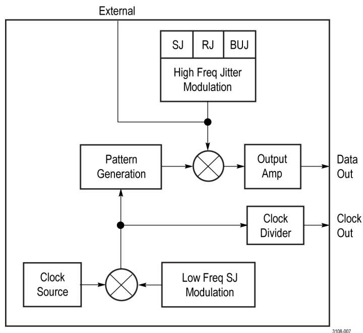
Figure 8: Jitter insertion block diagram
