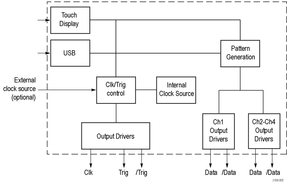
Figure 6: Block diagram
