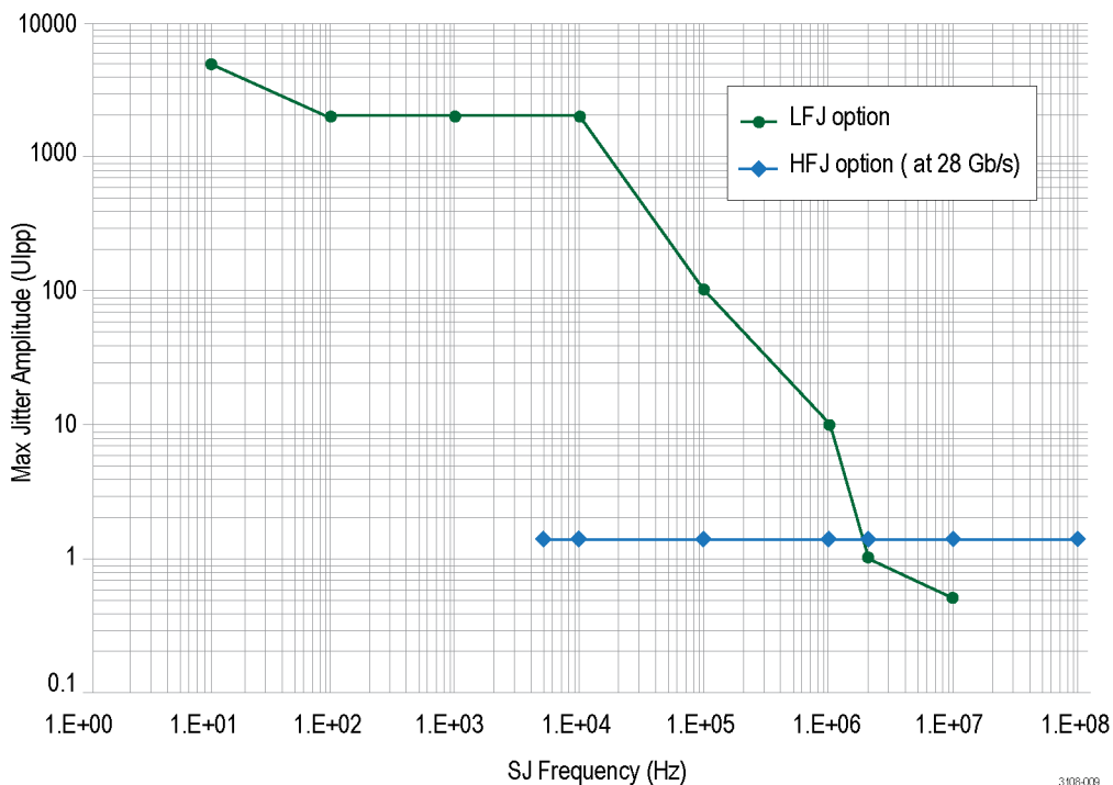
Figure 9: Low frequency (Option LFJIT) and high frequency (Option HFJIT) jitter insertion rates, based on a data rate of 28 Gb/s
