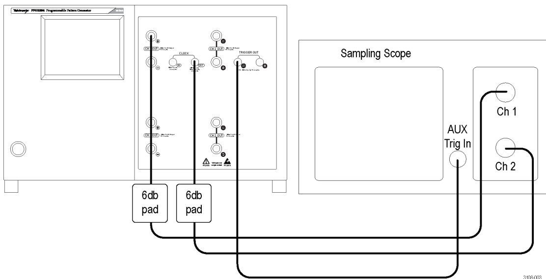
Figure 3: Verification setup
