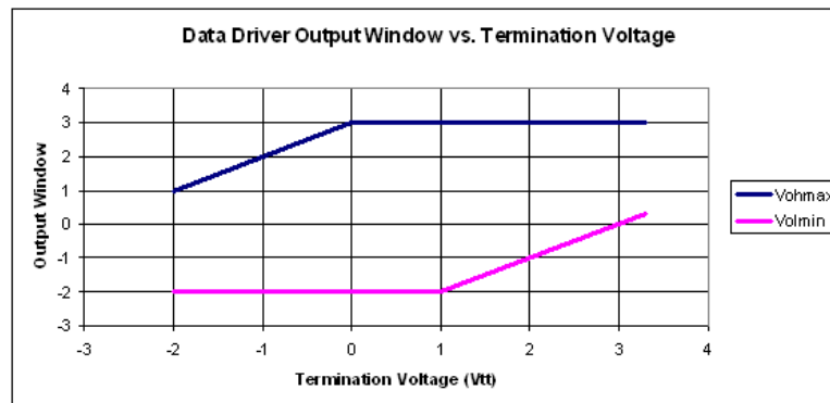
Figure 7: Available output range (PPG1600, PPG3000, and PPG3200 with ADJ option)
