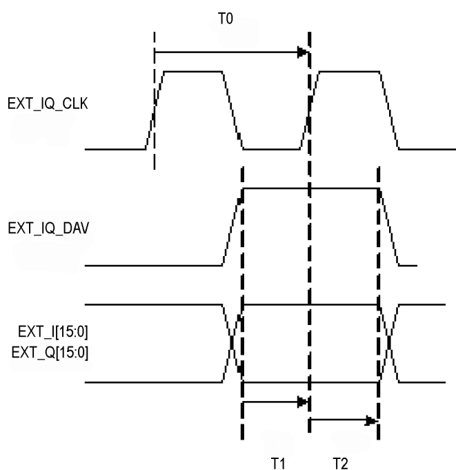
Figure 2: IQ Timing
