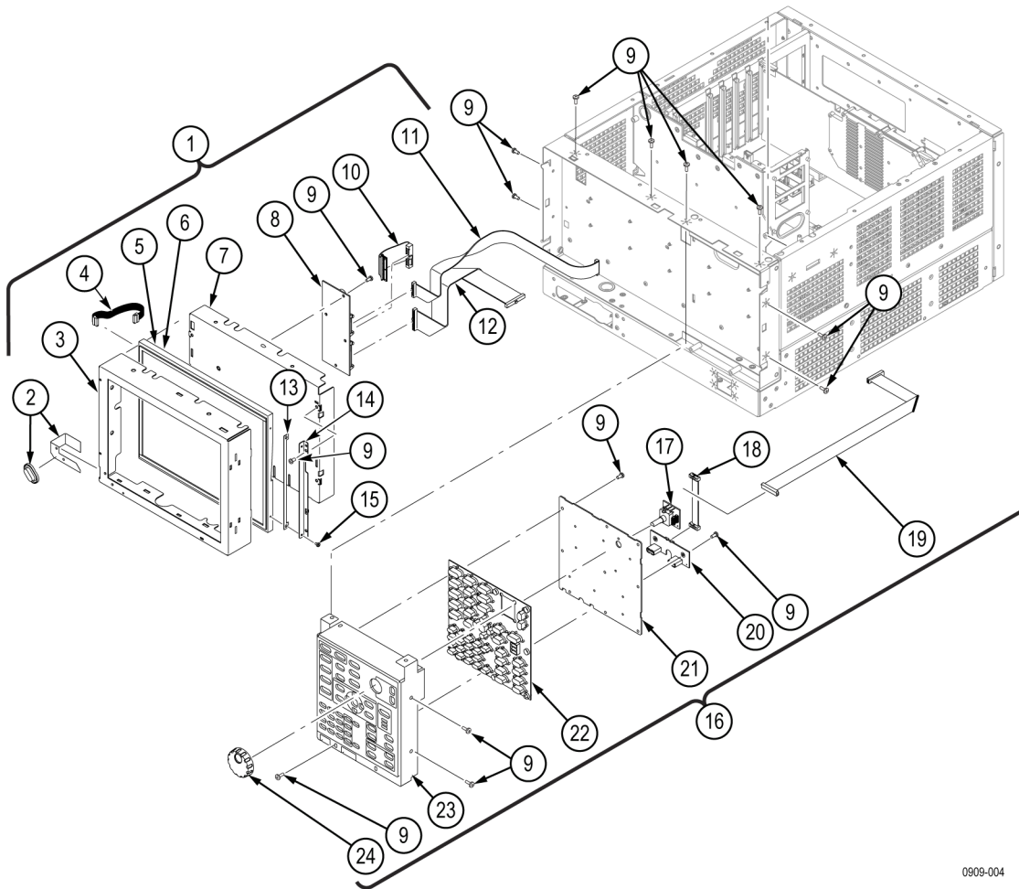
Figure 6: Display and front panel
