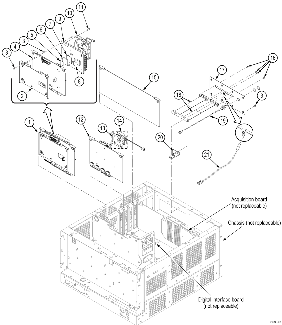
Figure 7: Modules
