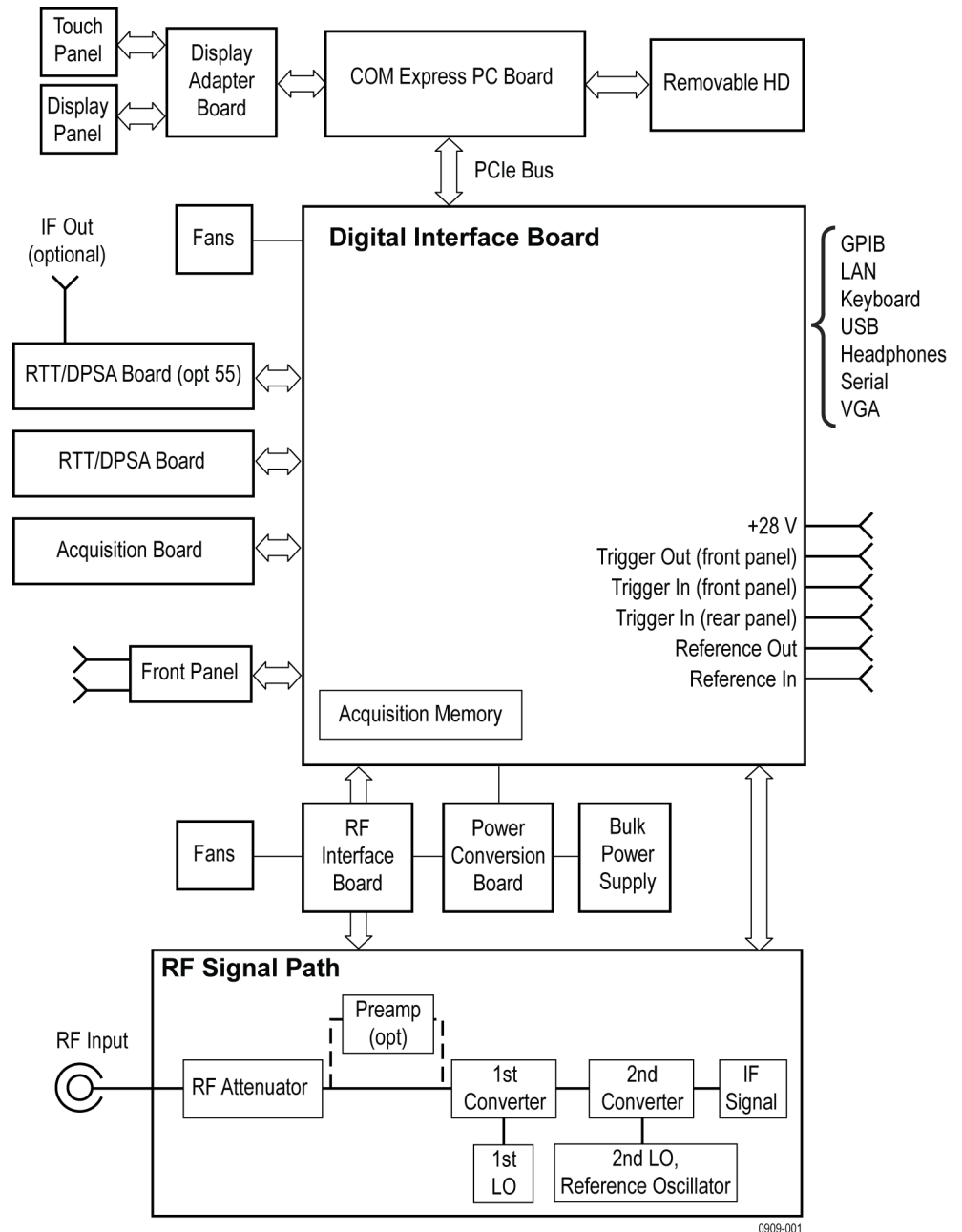
Figure 1: Block diagram
