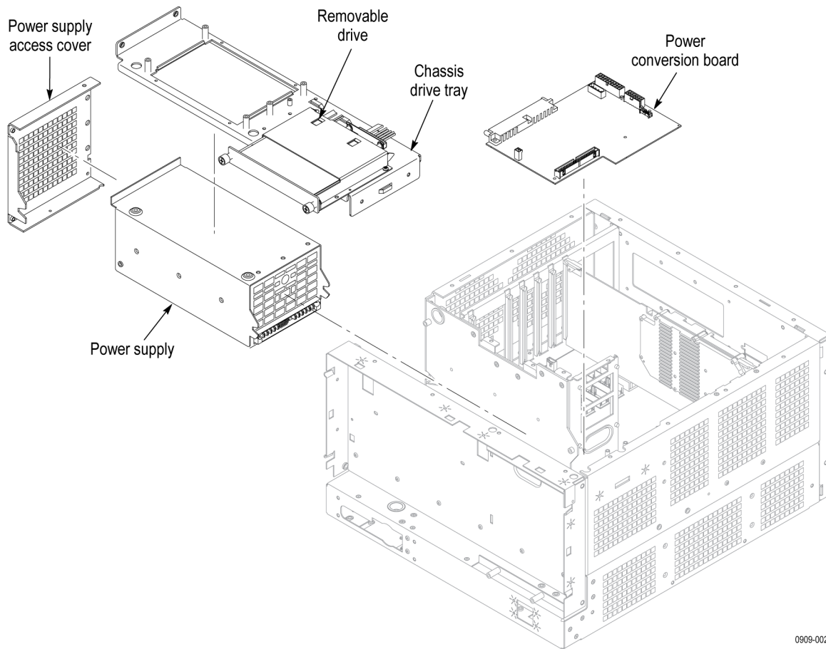
Figure 2: Power supply and HDD drive locations
