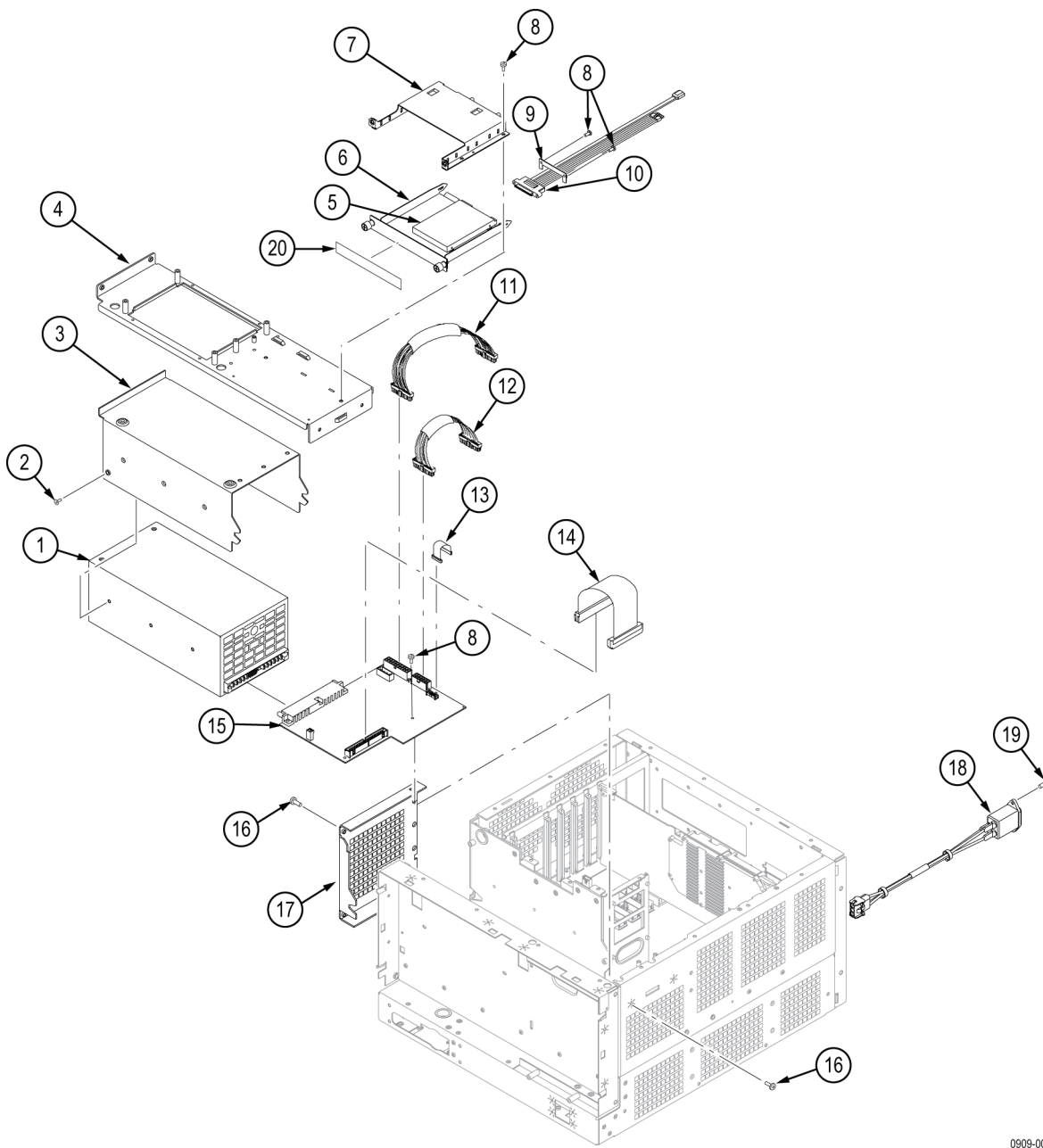
Figure 8: Power supply and removable hard drive
