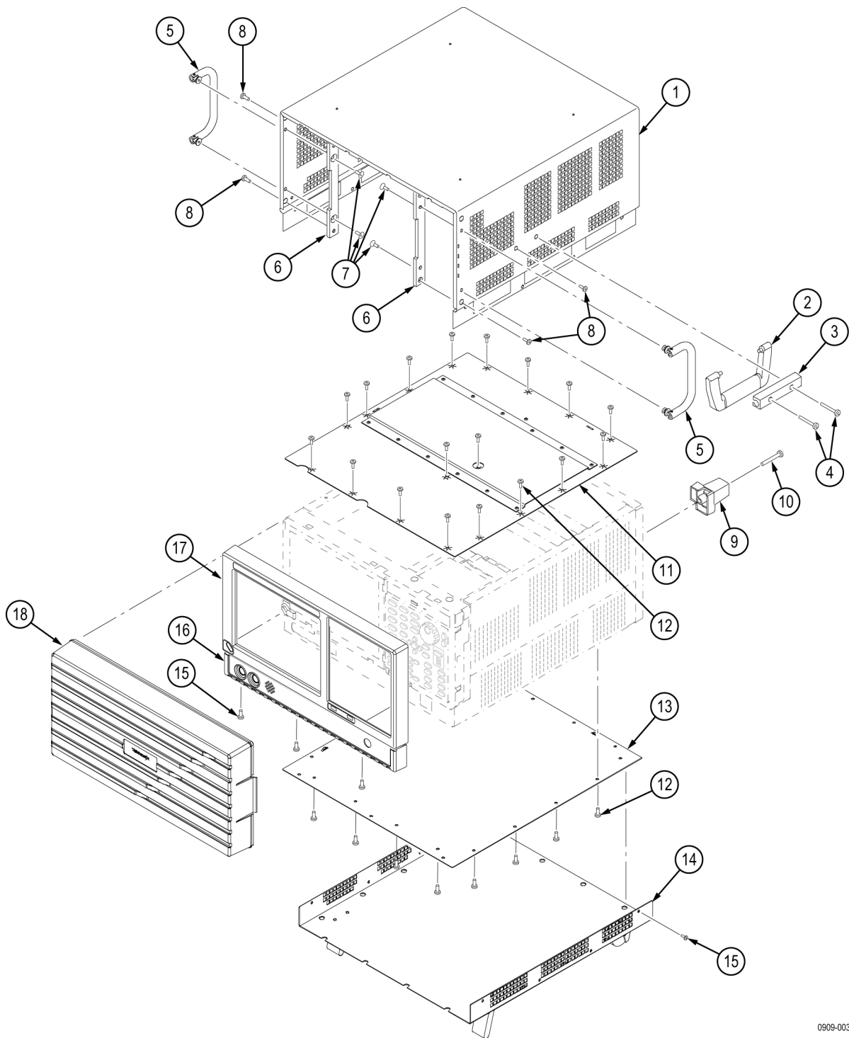
Figure 5: External parts
