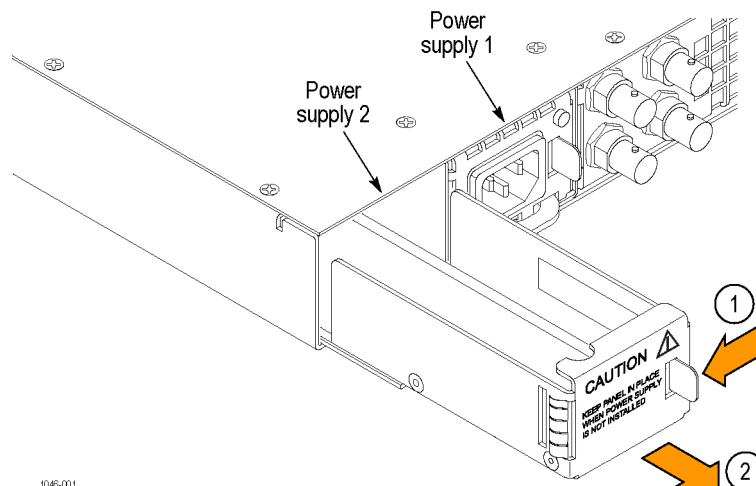
Figure 1: Removing the shield from the Power Supply 2 slot
