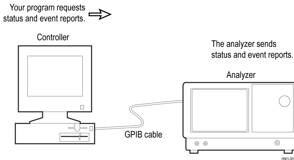
Figure 3: Event-driven program
