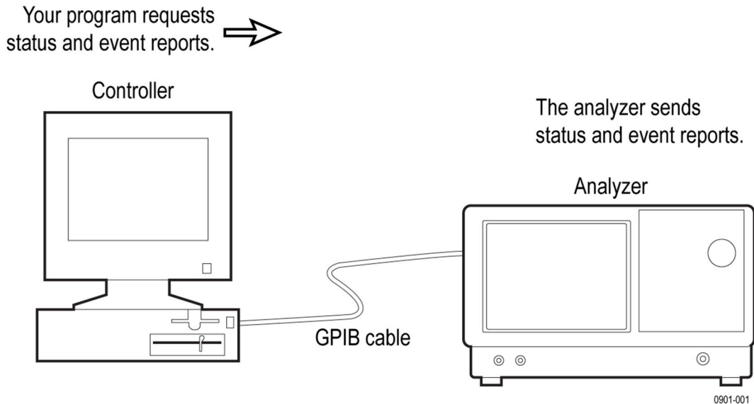
Event-driven program
