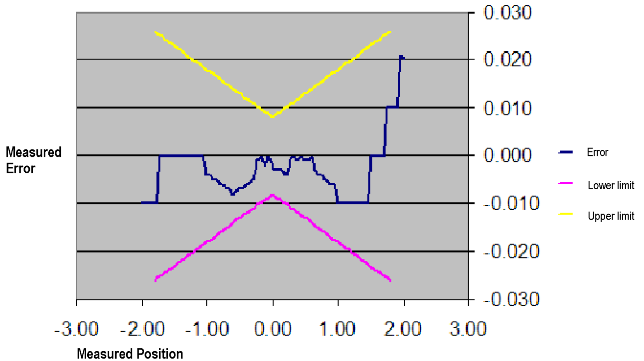
Figure 1: Example of a line graph for the Vertical Position Accuracy test
