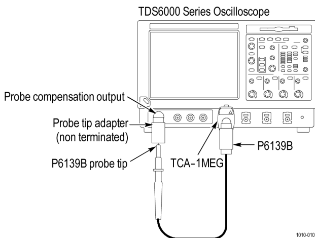
Figure 7: Setup with the P6139B attached to the TCA-1MEG
