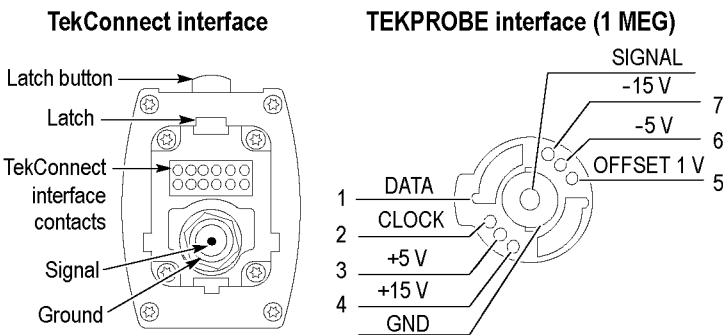
Figure 4: TekConnect and TEKPROBE Interface features
