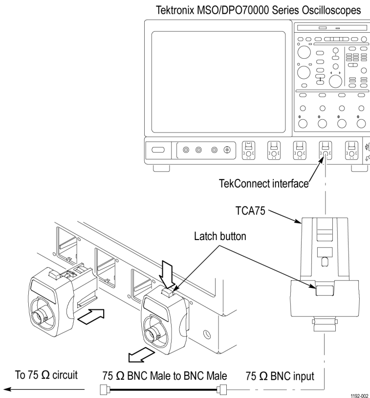
Figure 2: Connecting the adapter to oscilloscopes with the TekConnect interface
