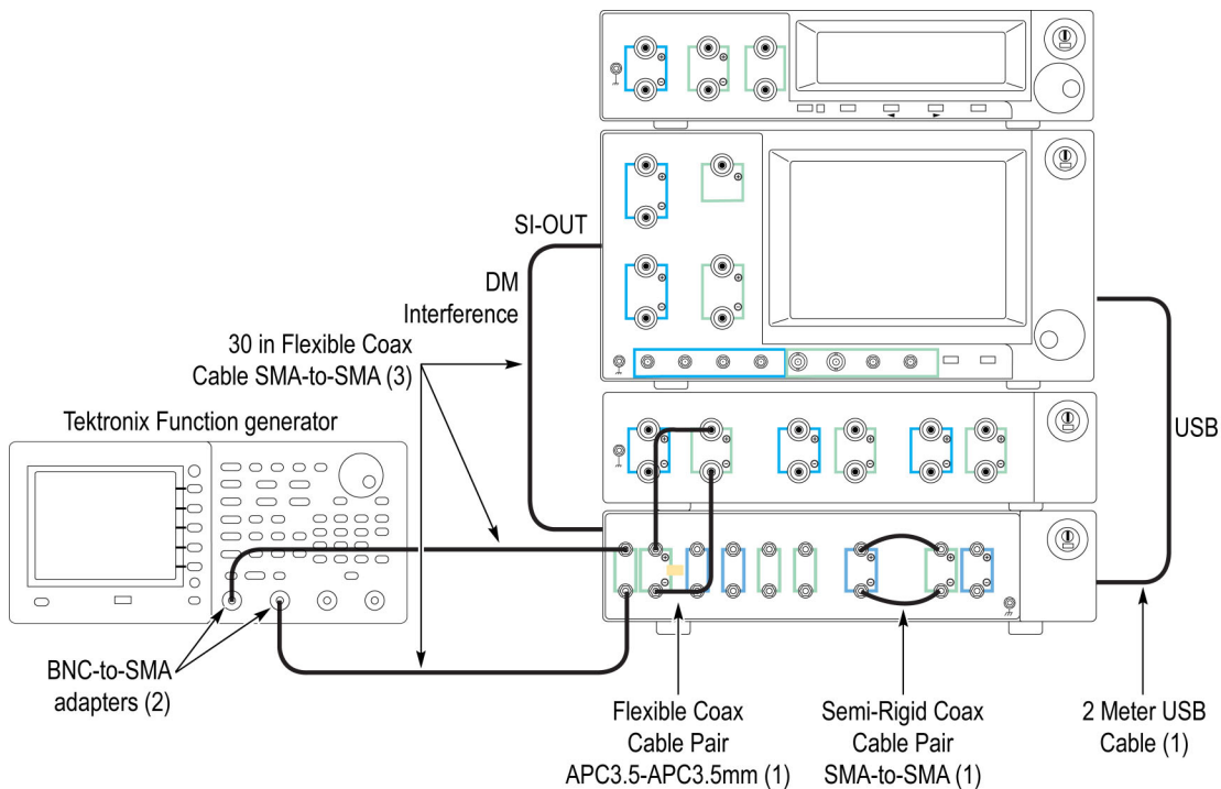
Figure 1: Sample configuration
