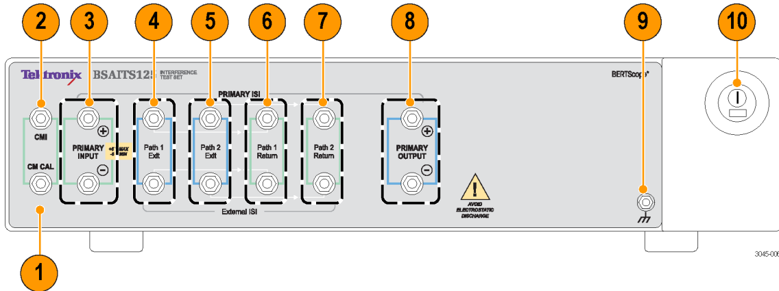
Figure 2: BSAITS125 front-panel connectors, standard instrument
