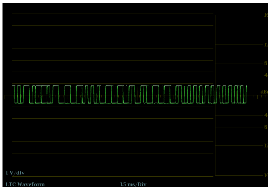
Figure 30: LTC Waveform display
