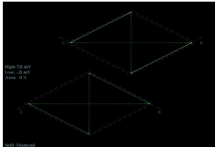
Figure 32: Split Diamond display
