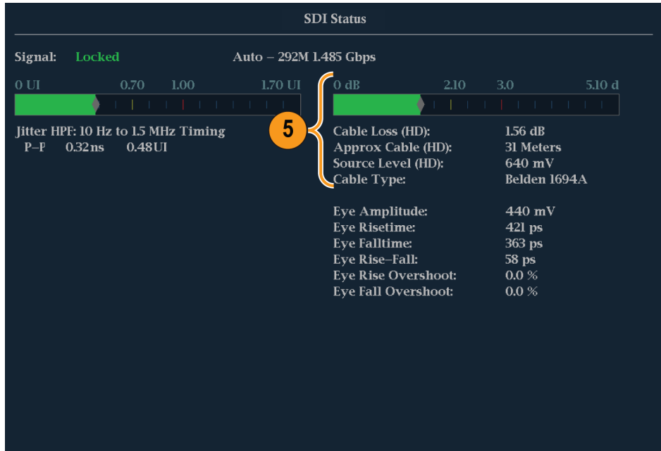
Figure 60: Cable loss information in the SDI Status display
