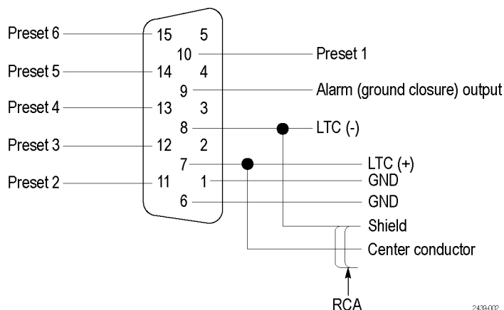
Figure 1: Wiring diagram for LTC input/Alarm (ground closure) output cable
