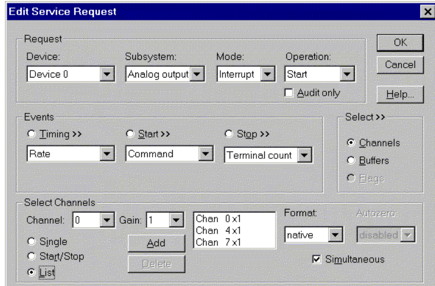
How to set up the KPCMCIA-8AO Series using a channel list to write to multiple DACs
