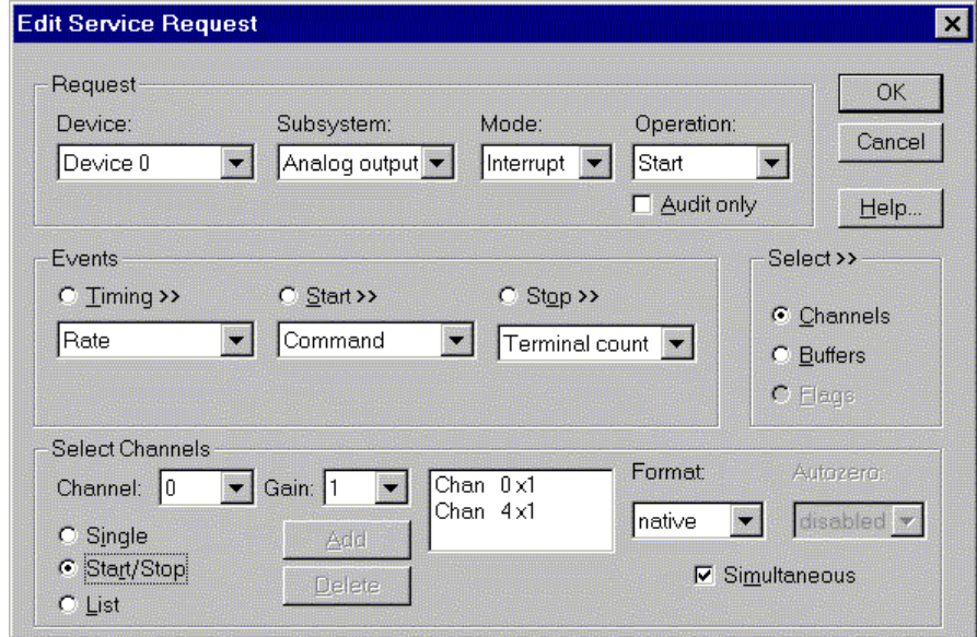
How to set up the KPCMCIA-8AO Series using a start/stop range to write to multiple DACs
