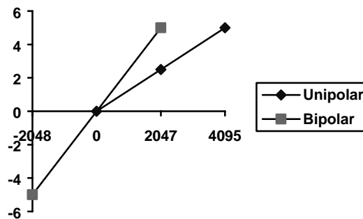
KPCMCI A-8AO Series native D/A Codes versus Voltage Range
