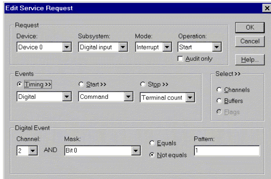
How to set up the KPCMCI A-8AO Series for external rate sampling using a digital event.
