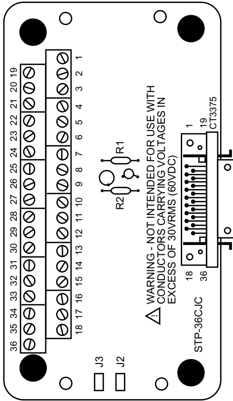
Figure 1 Pin connections
